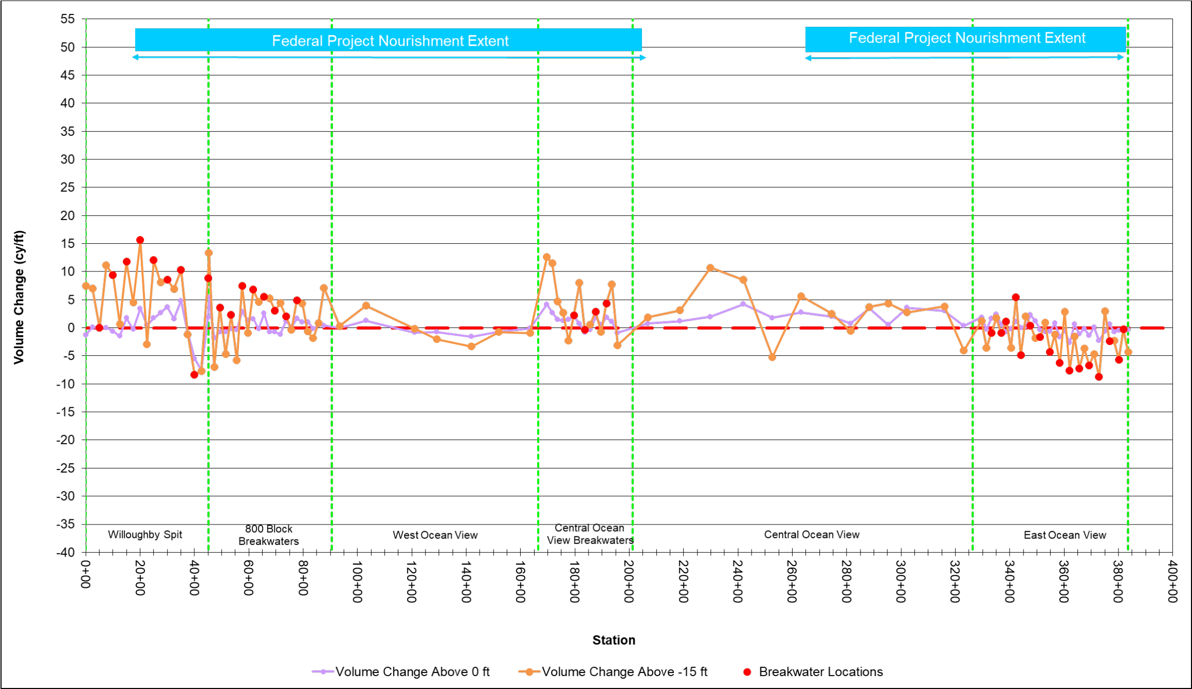
Figure 5-17: Volume Change above 0 ft NAVD88 and -15 ft NAVD88 (cy/ft) for November 2022 to May 2023 (Note: Positive = Accretion, Negative = Erosion)
