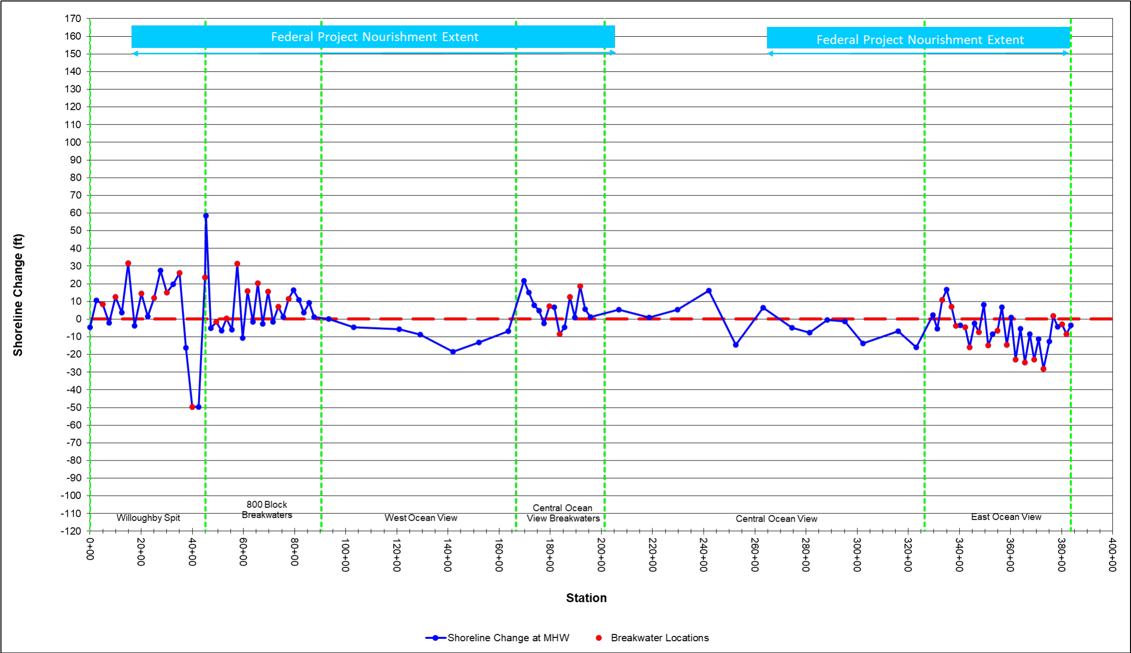
Figure 5-16: Shoreline Change (ft) at Mean High Water (+0.98 ft NAVD88) for November 2022 to May 2023 (Note: Positive = Accretion, Negative = Erosion)
