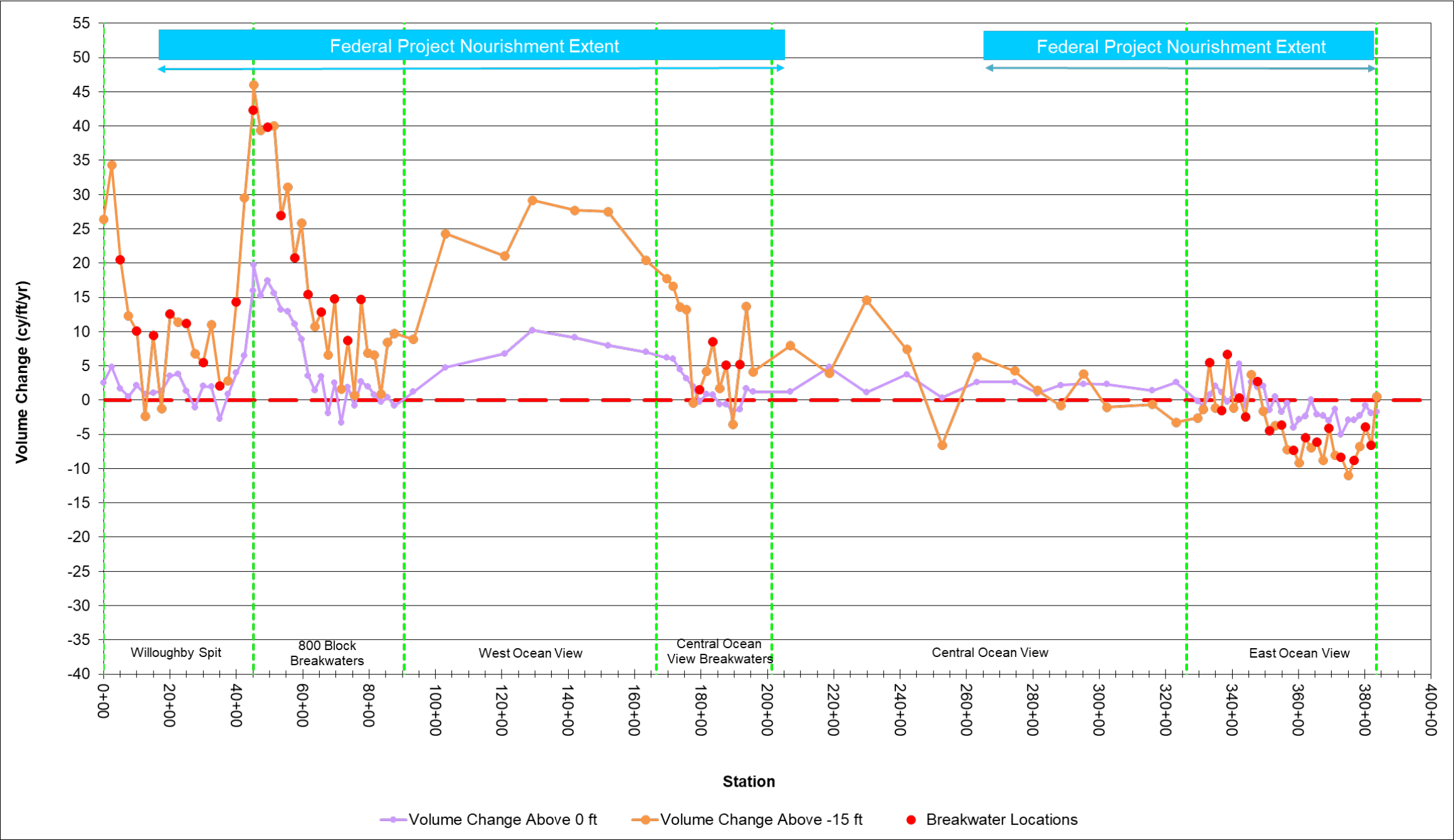
Figure 5-15: Volume Change Rate Above 0 ft NAVD88 and -15 ft NAVD88 (cy/ft/yr) for April 2022 to May 2023 (Note: Positive = Accretion, Negative = Erosion)
