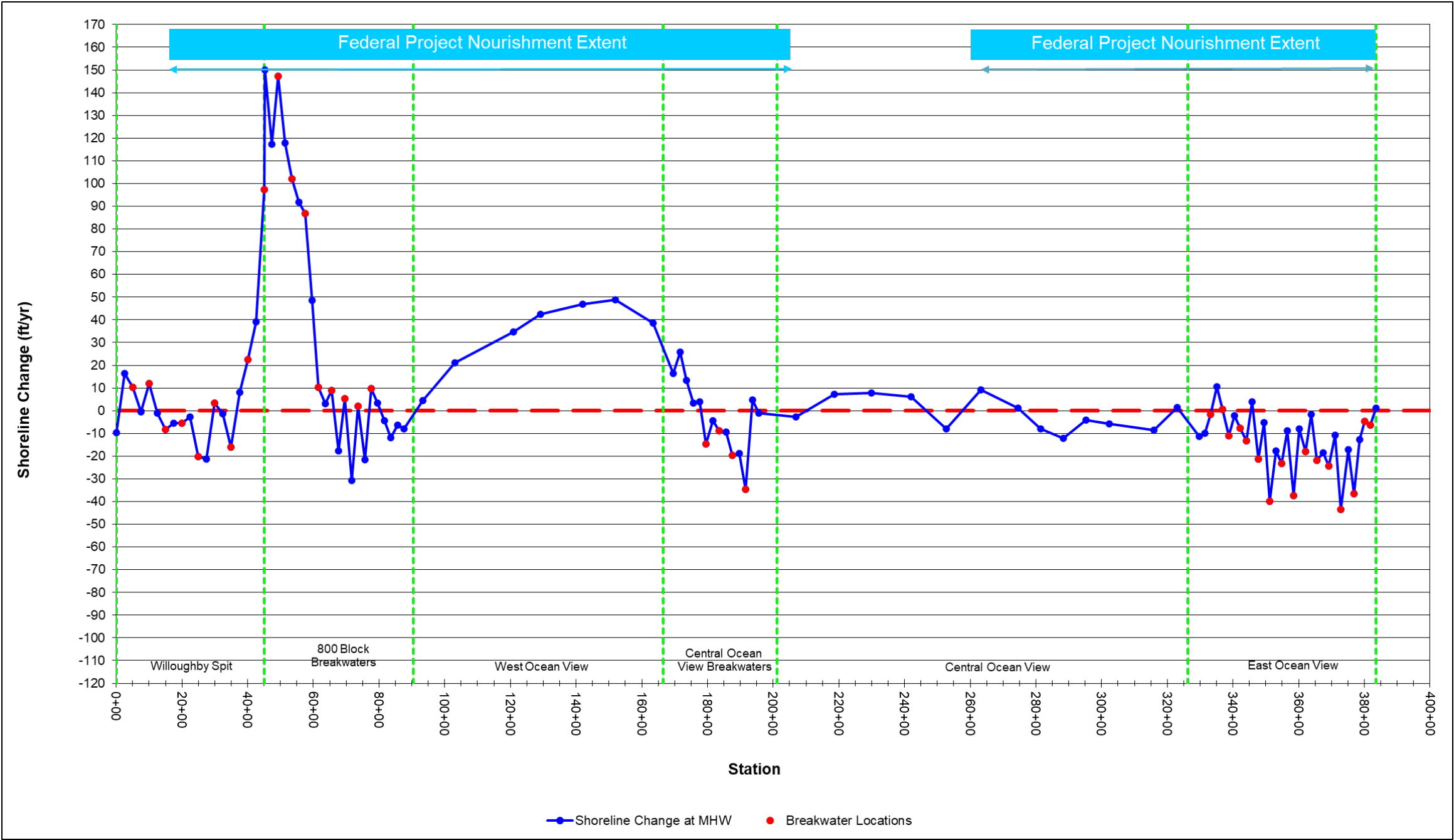
Figure 5-14: Shoreline Change Rate (ft/yr) at Mean High Water (+0.98 ft NAVD88) for April 2022 to May 2023 (Note: Positive = Accretion, Negative = Erosion)
