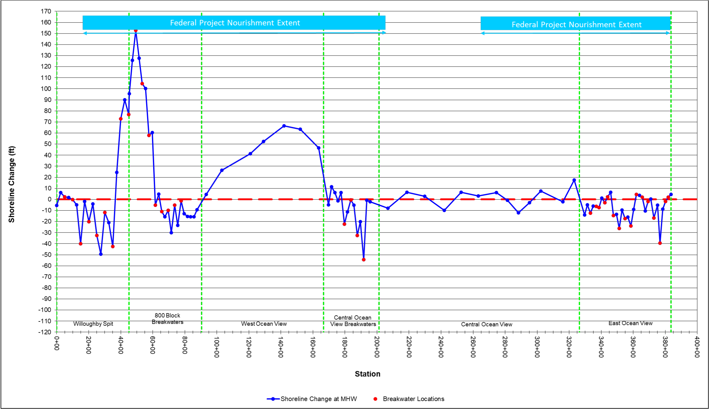
Figure 5-16: Shoreline Change (ft) at Mean High Water (+0.98 ft NAVD88) for April 2022 to November 2022 (Note: Positive = Accretion, Negative = Erosion)
