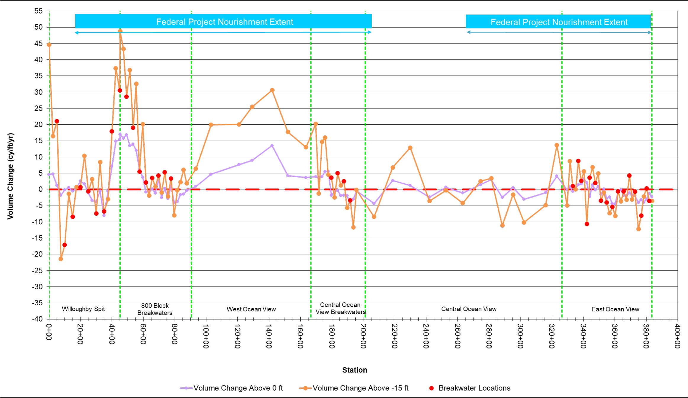
Figure 5-15: Volume Change Rate Above 0 ft NAVD88 and -15 ft NAVD88 (cy/ft/yr) for October 2021 to November 2022 (Note: Positive = Accretion, Negative = Erosion)
