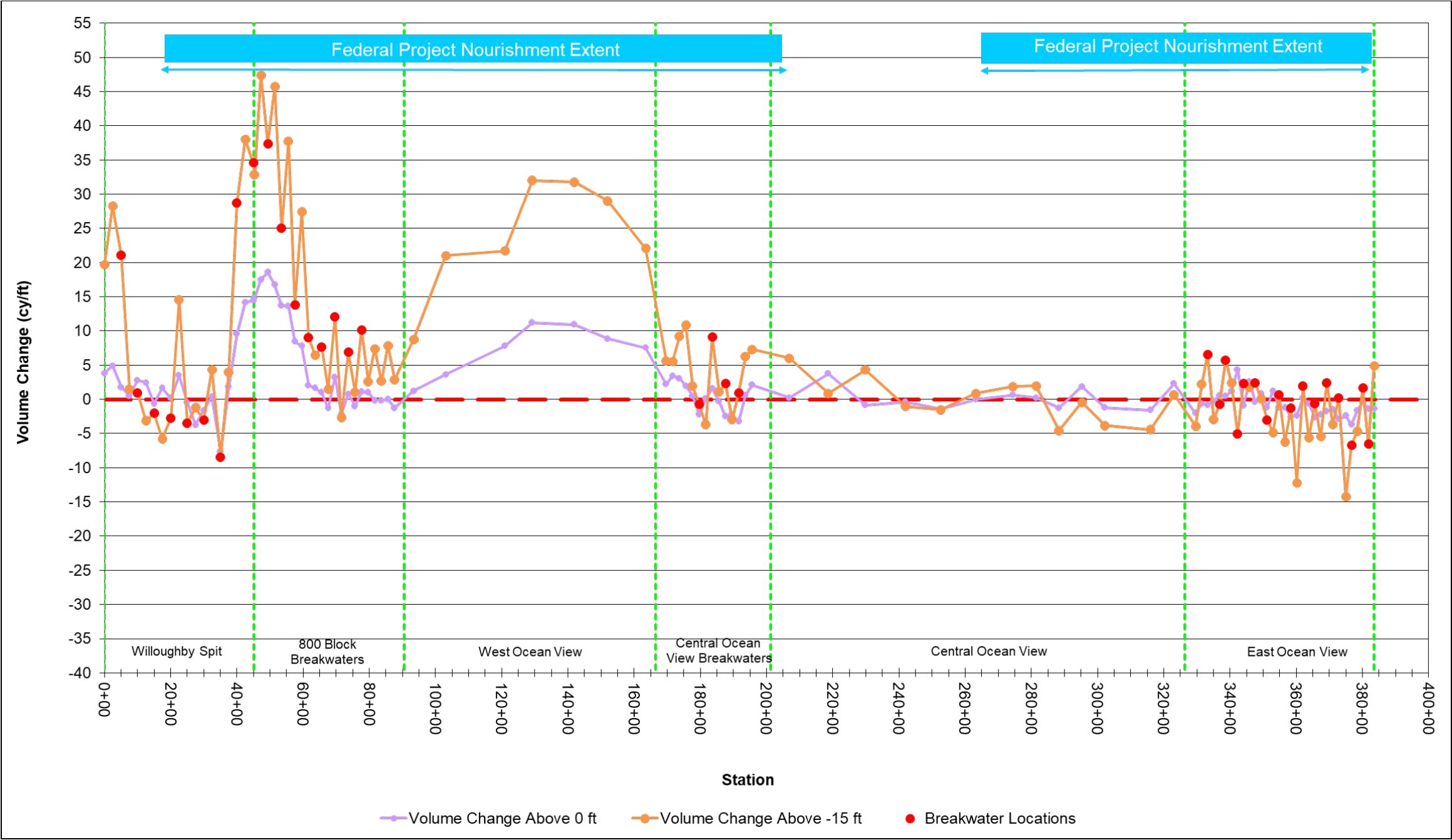
Figure 5-17: Volume Change above 0 ft NAVD88 and -15 ft NAVD88 (cy/ft) for April 2022 to November 2022 (Note: Positive = Accretion, Negative = Erosion)
