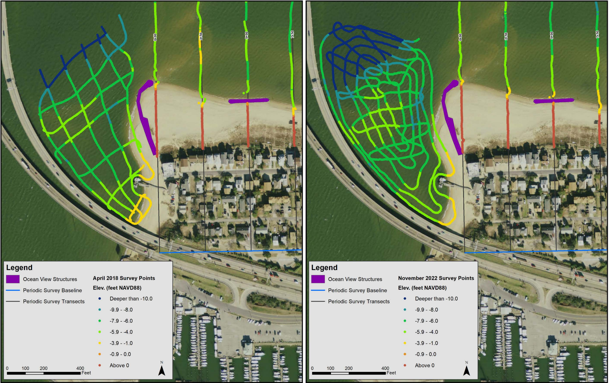
Figure 6-1: Spring 2018 and Fall 2022 Survey Depths West of the Willoughby Spit Terminal Groin
