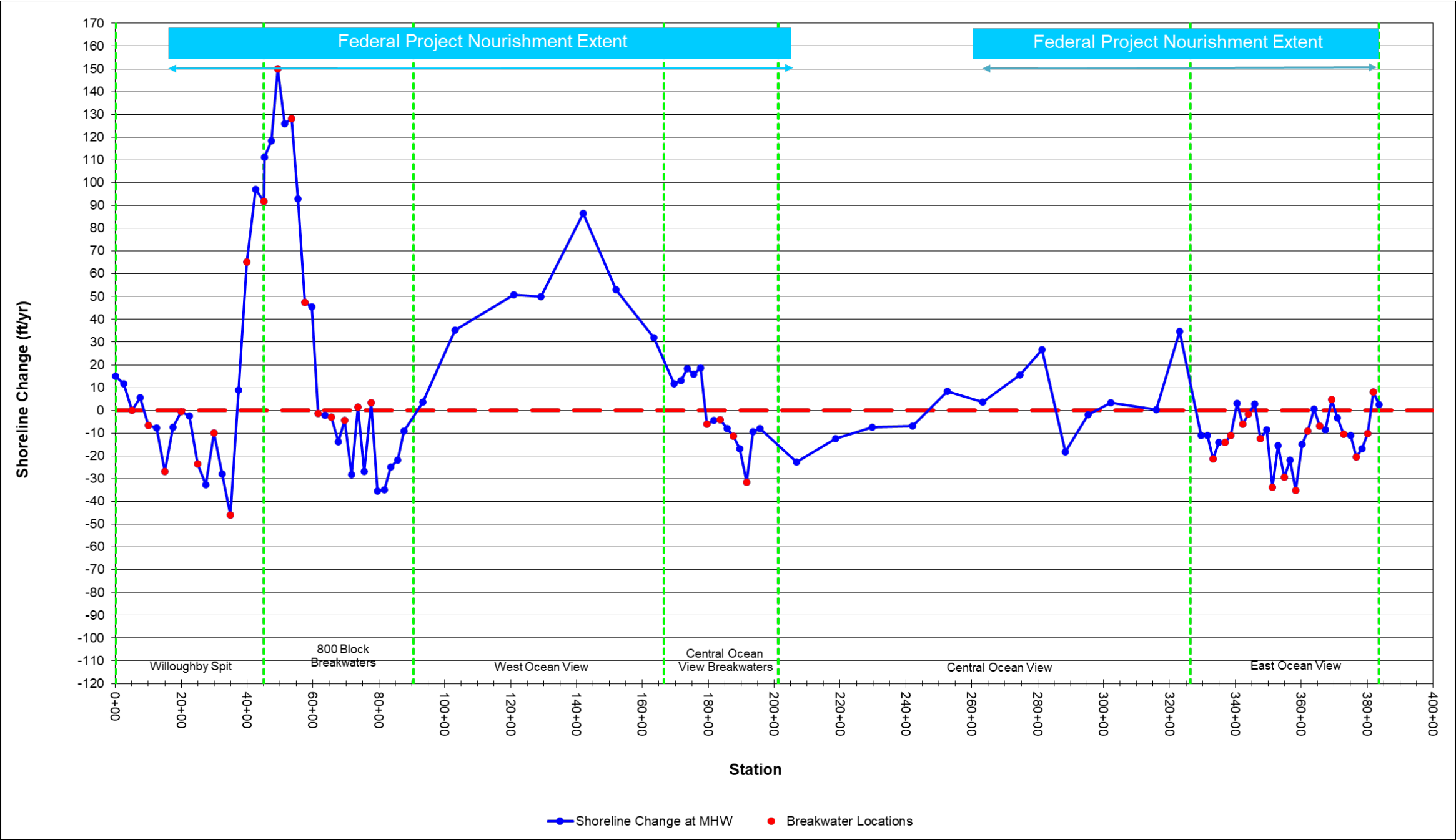
Figure 5-14: Shoreline Change Rate (ft/yr) at Mean High Water (+0.98 ft NAVD88) for October 2021 to November 2022 (Note: Positive = Accretion, Negative = Erosion)
