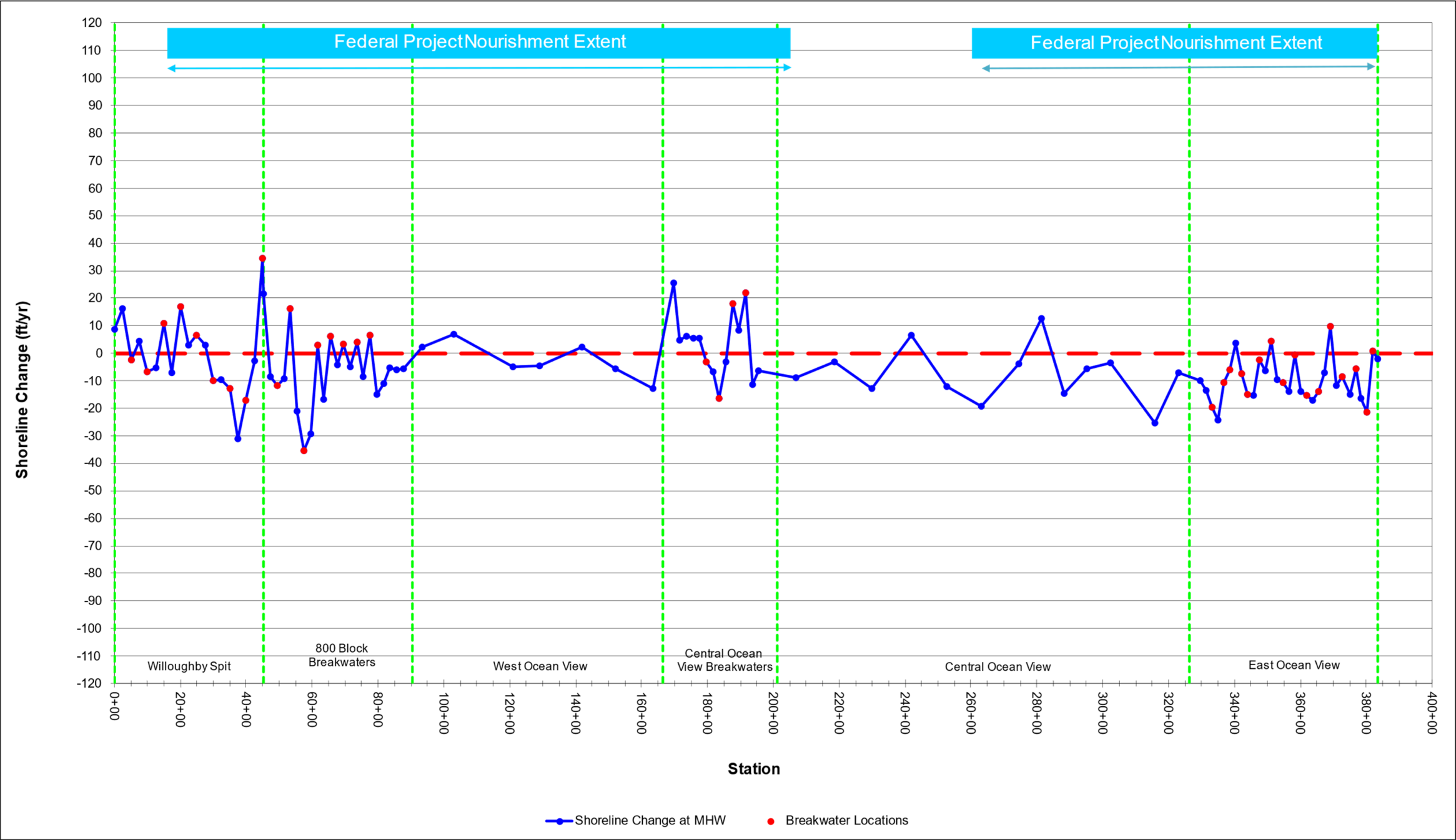
Figure 5-25: Shoreline Change Rate (ft/yr) at Mean High Water (+0.98 ft NAVD88) for June 2021 to April 2022 (Note: Positive = Accretion, Negative = Erosion)
