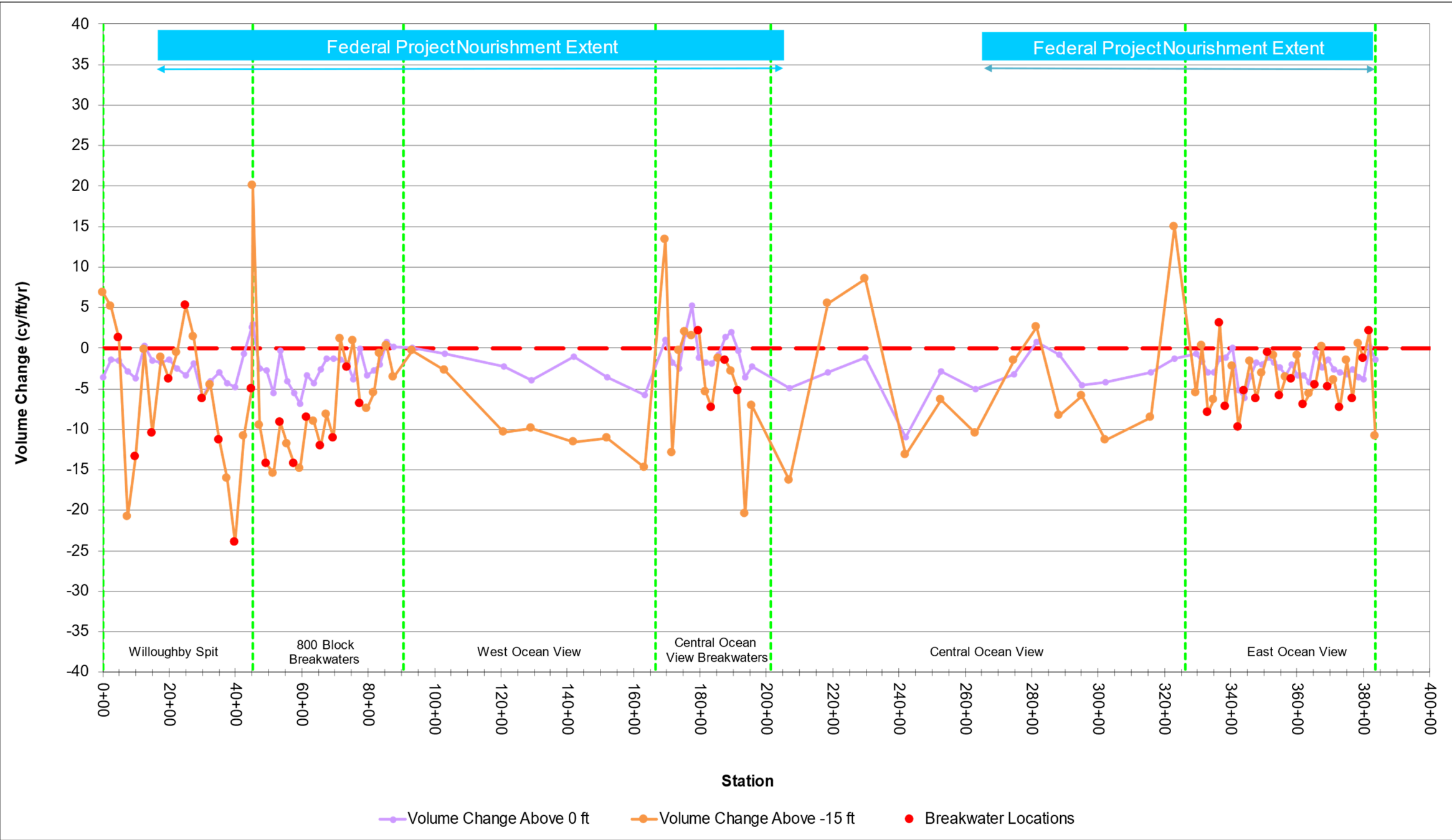
Figure 5-26: Volume Change Rate Above 0 ft NAVD88 and -15 ft NAVD88 (cy/ft/yr) for June 2021 to April 2022 (Note: Positive = Accretion, Negative = Erosion)
