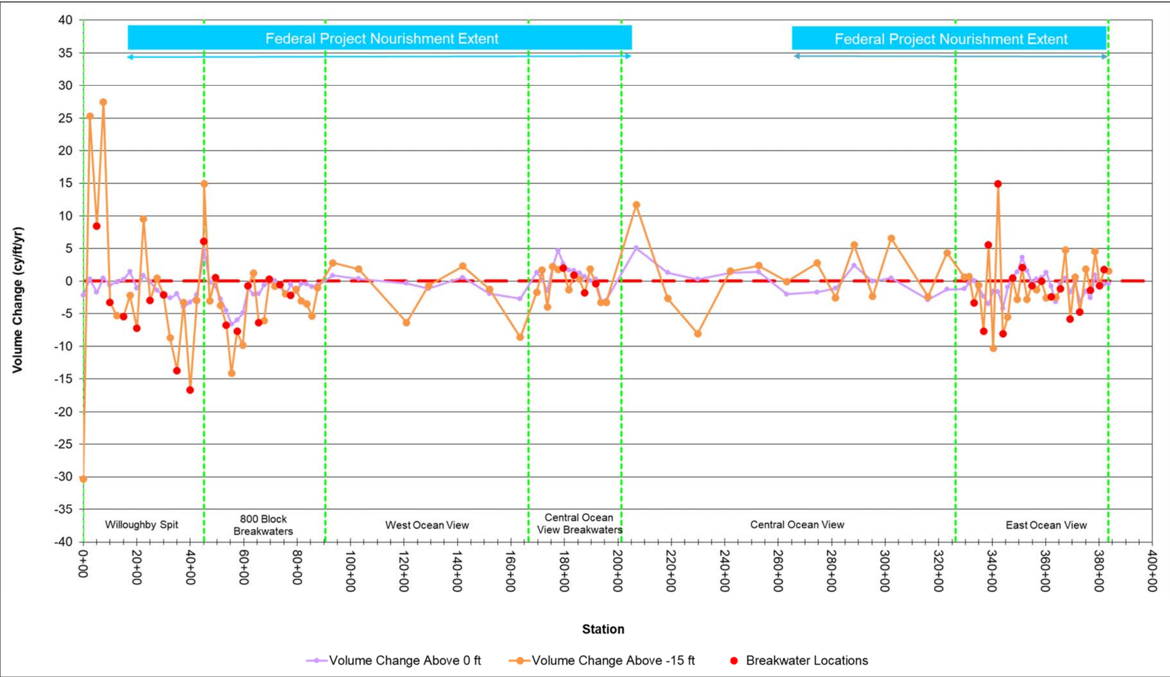
Figure 5-41: Volume Change Rate Above 0 ft NAVD88 and -15 ft NAVD88 (cy/ft/yr) for October 2020 to October 2021 (Note: Positive = Accretion, Negative = Erosion)
