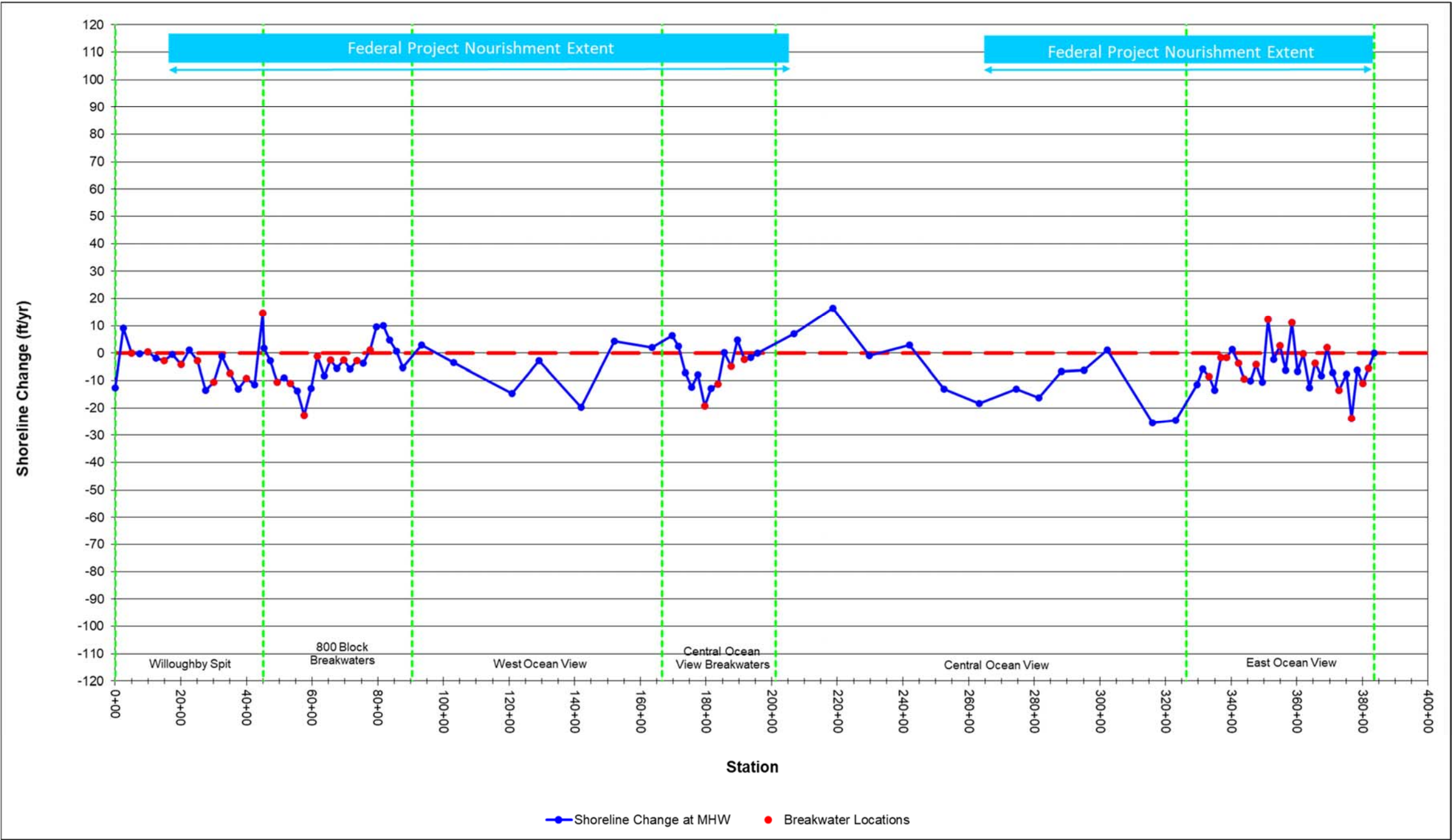
Figure 5-42: Shoreline Change (ft) at Mean High Water (+0.98 ft NAVD88) for June 2021 to October 2021 (Note: Positive = Accretion, Negative = Erosion)
