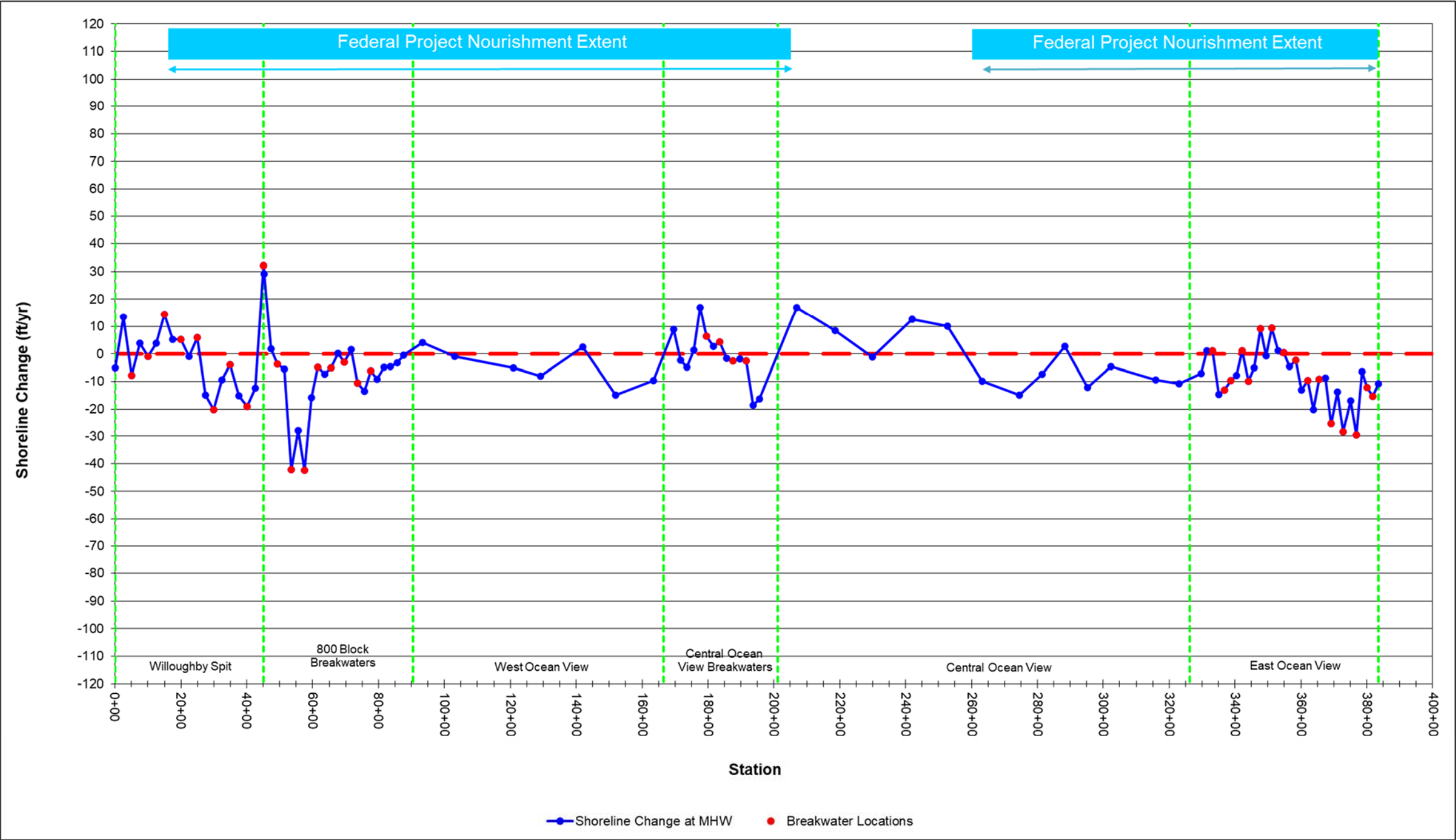
Figure 5-40: Shoreline Change Rate (ft/yr) at Mean High Water (+0.98 ft NAVD88) for October 2020 to October 2021 (Note: Positive = Accretion, Negative = Erosion)
