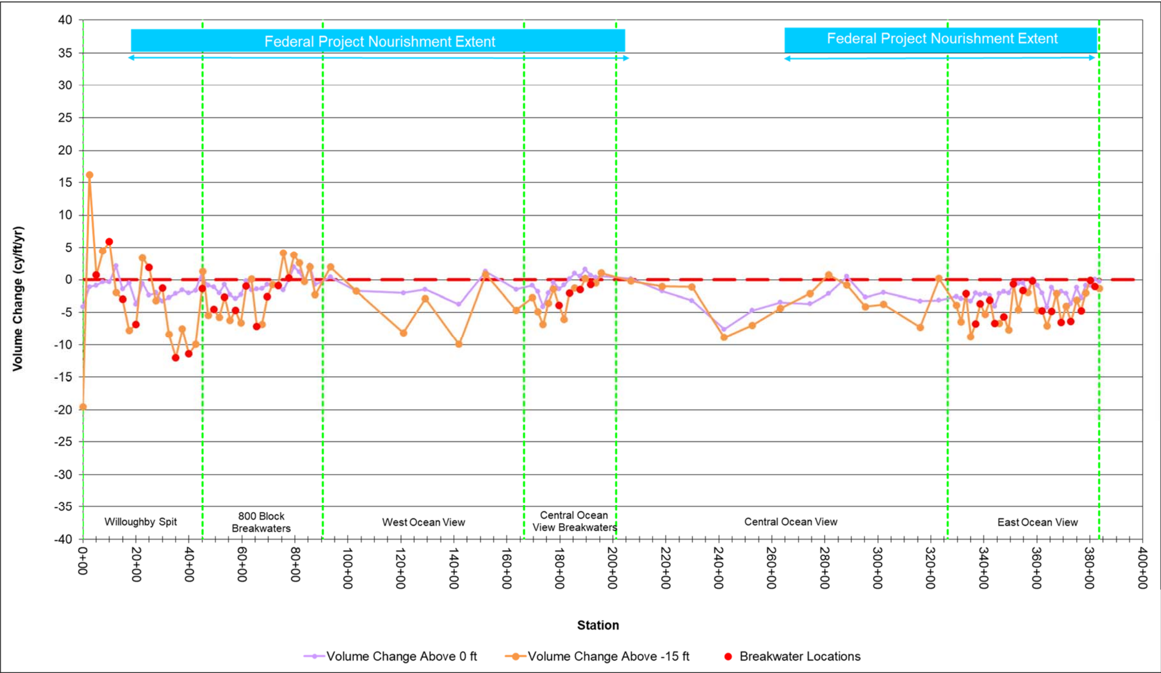
Figure 5-43: Volume Change above 0 ft NAVD88 and -15 ft NAVD88 (cy/ft) for June 2021 to October 2021 (Note: Positive = Accretion, Negative = Erosion)
