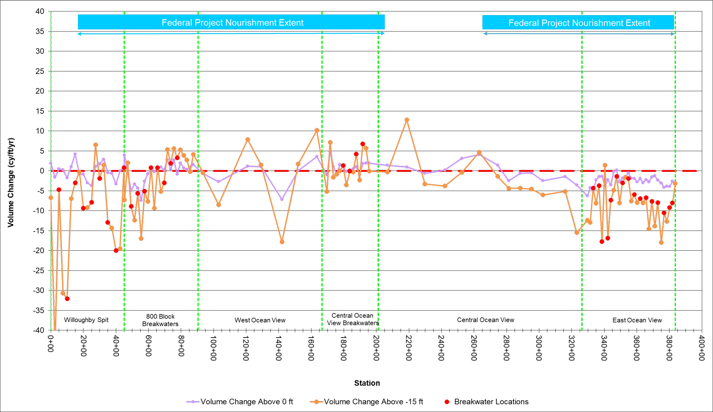
Figure 5-35: Volume Change Rate Above 0 ft NAVD88 and -15 ft NAVD88 (cy/ft/yr) for November 2019 to October 2020 (Note: Positive = Accretion, Negative = Erosion)
