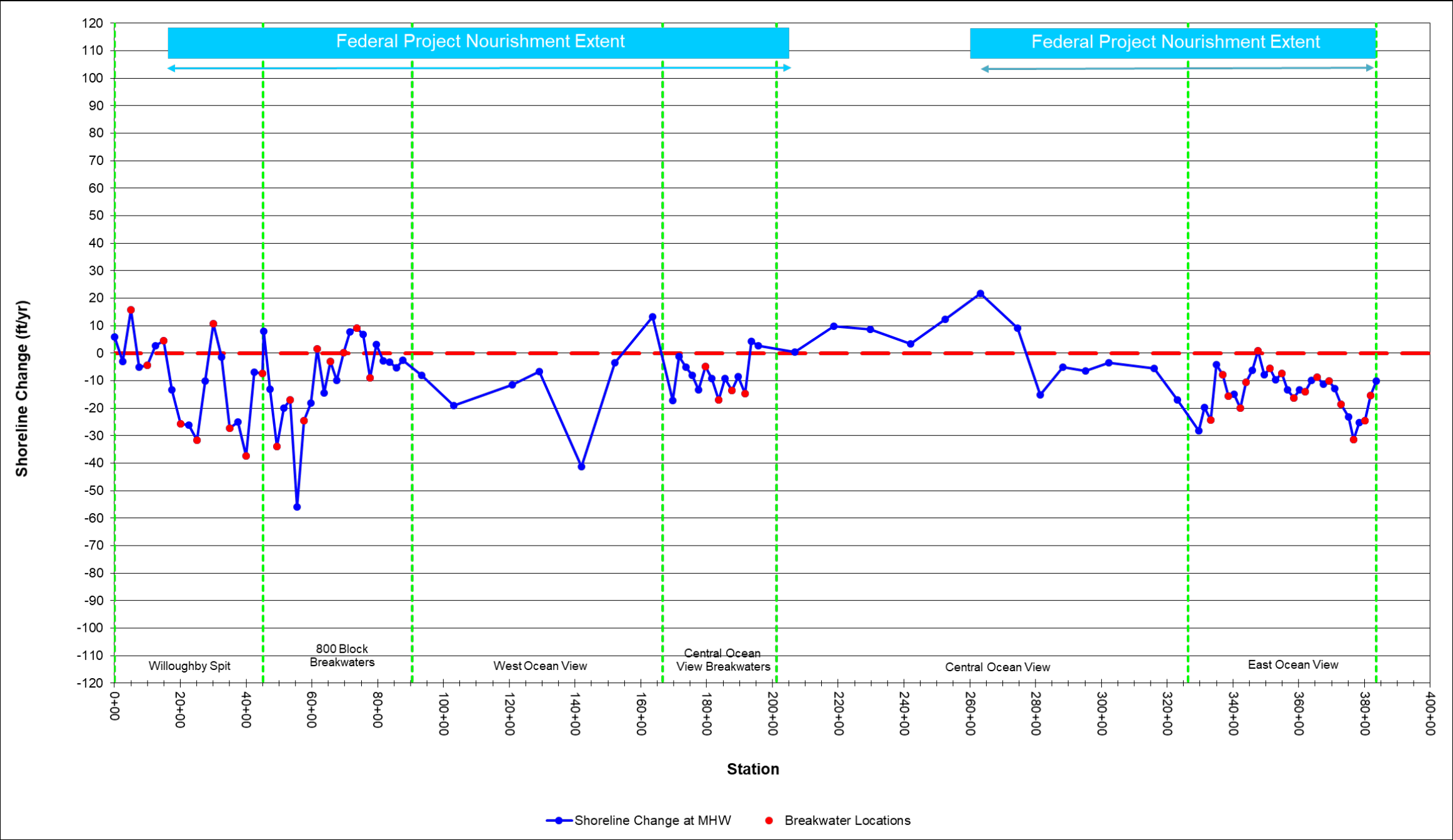
Figure 5-34: Shoreline Change Rate (ft/yr) at Mean High Water (+0.98 ft NAVD88) for November 2019 to October 2020 (Note: Positive = Accretion, Negative = Erosion)
