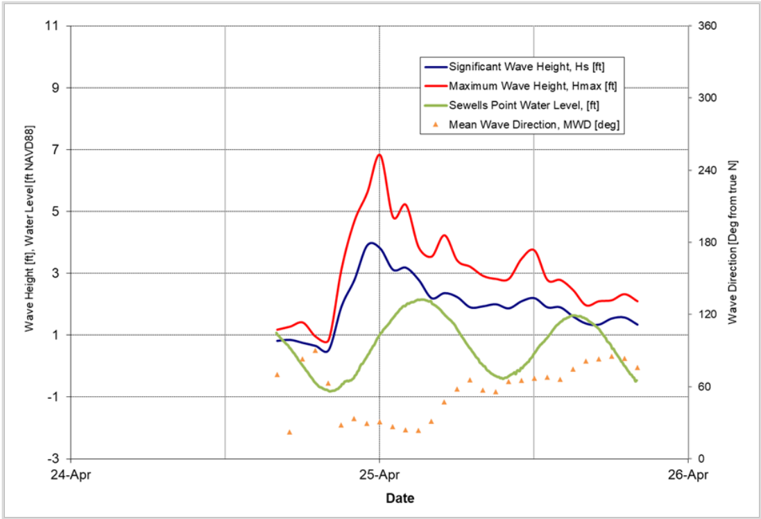
Figure 5-17: April 24, 2020 Storm
