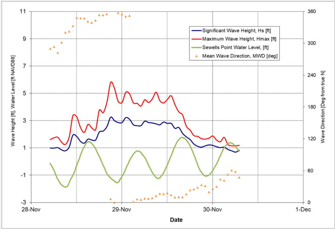
Figure 5-5: November 28, 2019 Storm
