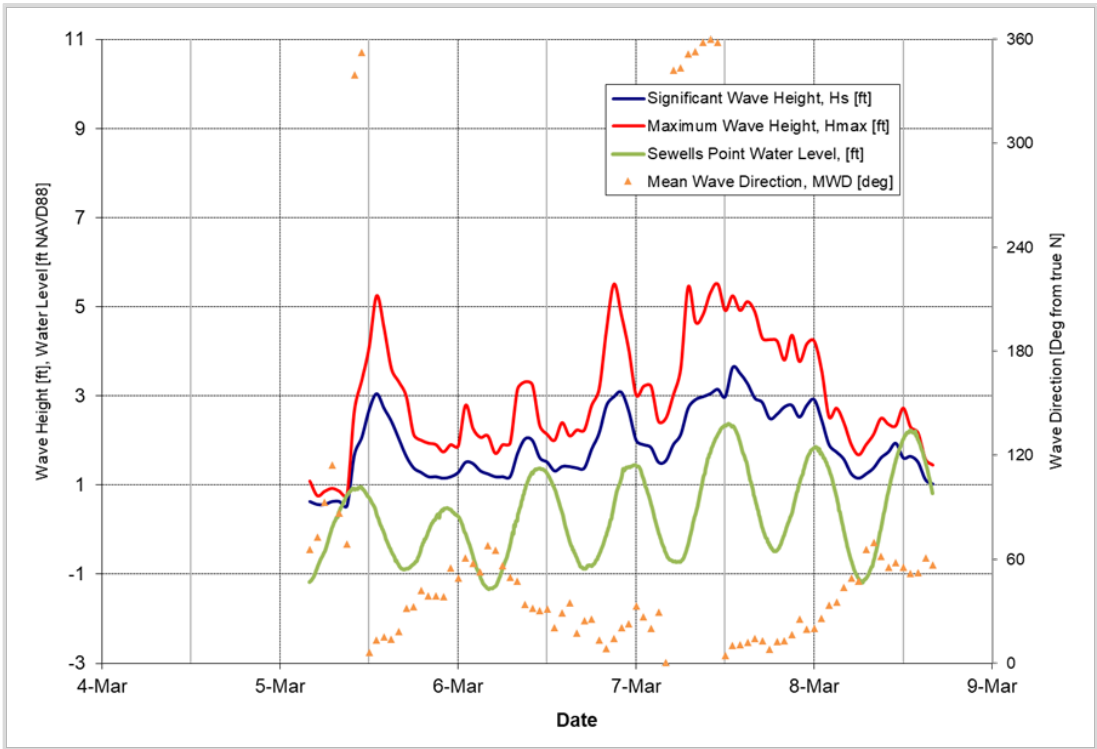
Figure 5-14: March 7, 2020 Storm
