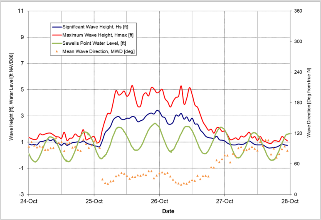
Figure 5-32: October 25, 2020 Storm
