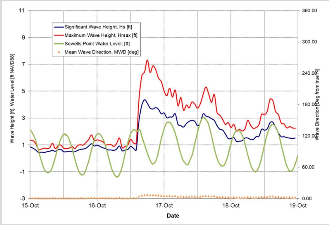
Figure 5-31: October 16, 2020 Storm
