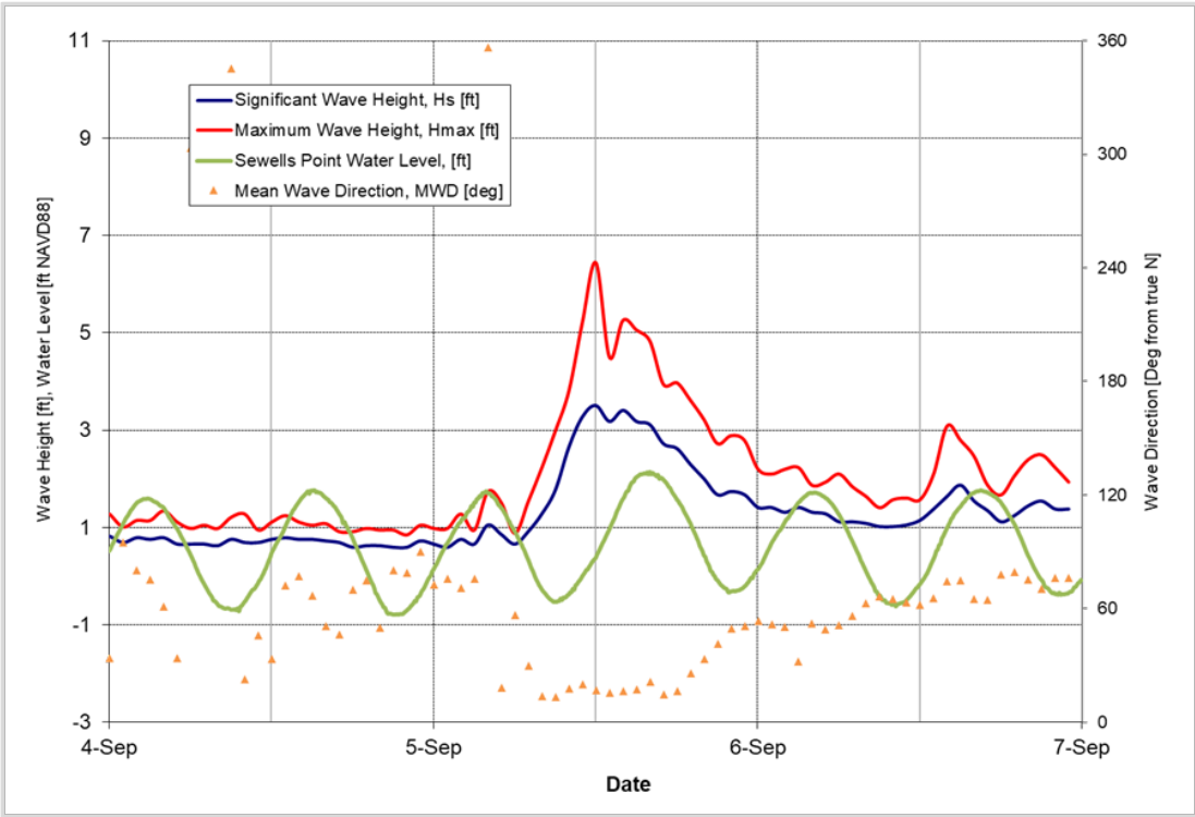
Figure 5-27: September 5, 2020 Storm
