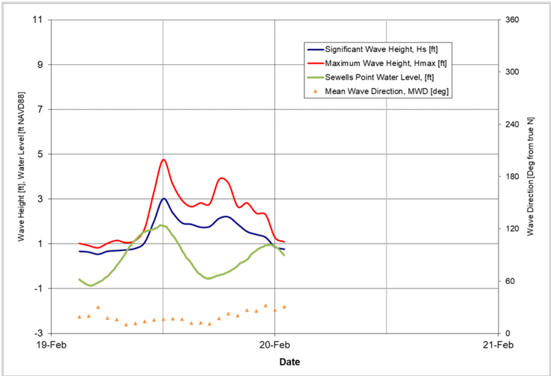
Figure 5-12: February 19, 2020 Storm
