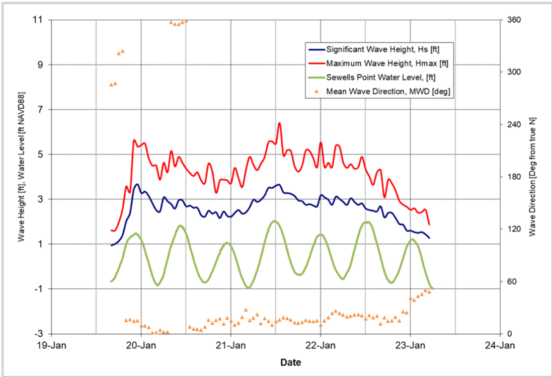
Figure 5-10: January 21, 2020 Storm
