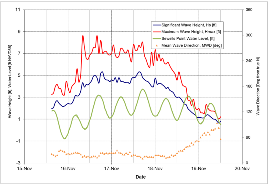
Figure 5-4: November 16, 2019 Storm
