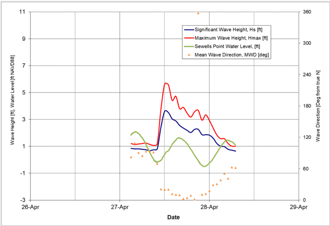
Figure 5-18: April 27, 2020 Storm
