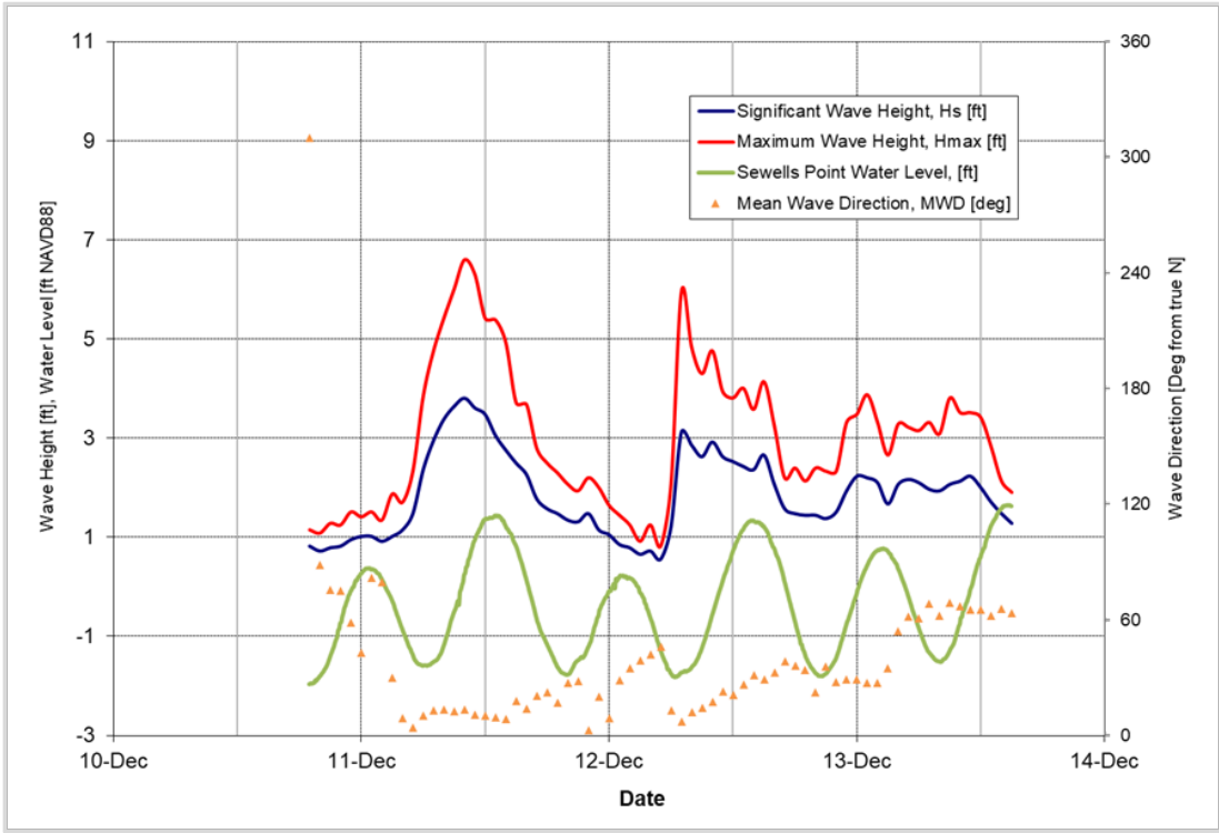
Figure 5-7: December 11, 2019 Storm
