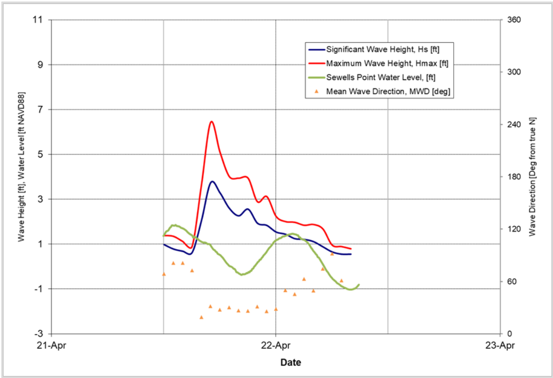
Figure 5-16: April 22, 2020 Storm
