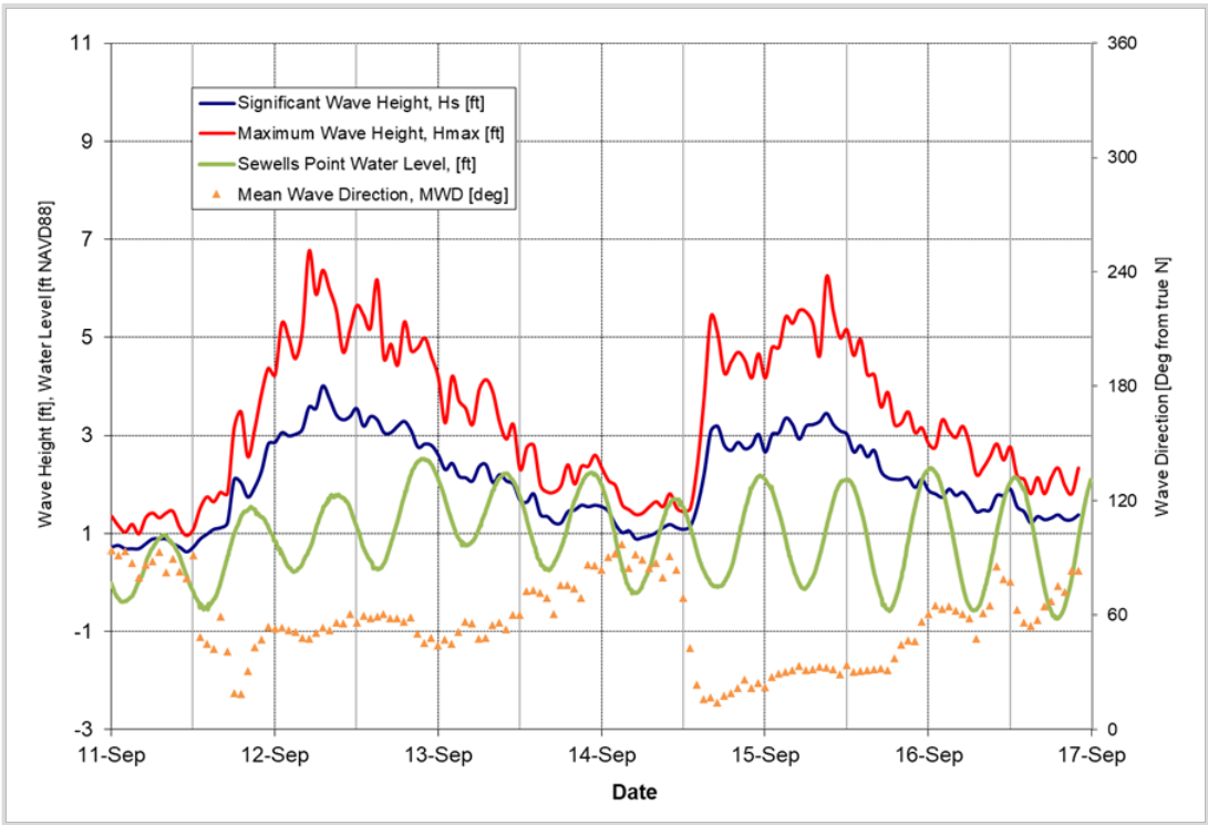
Figure 5-28: September 12, 2020 Storm
