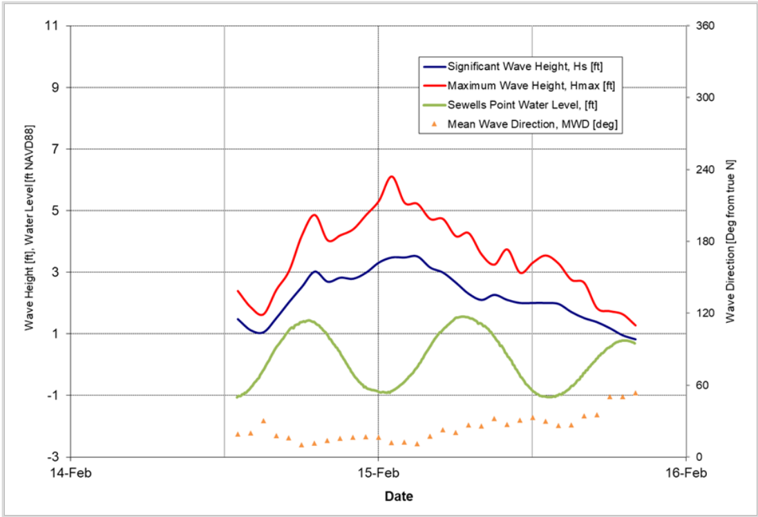
Figure 5-11: February 15, 2020 Storm
