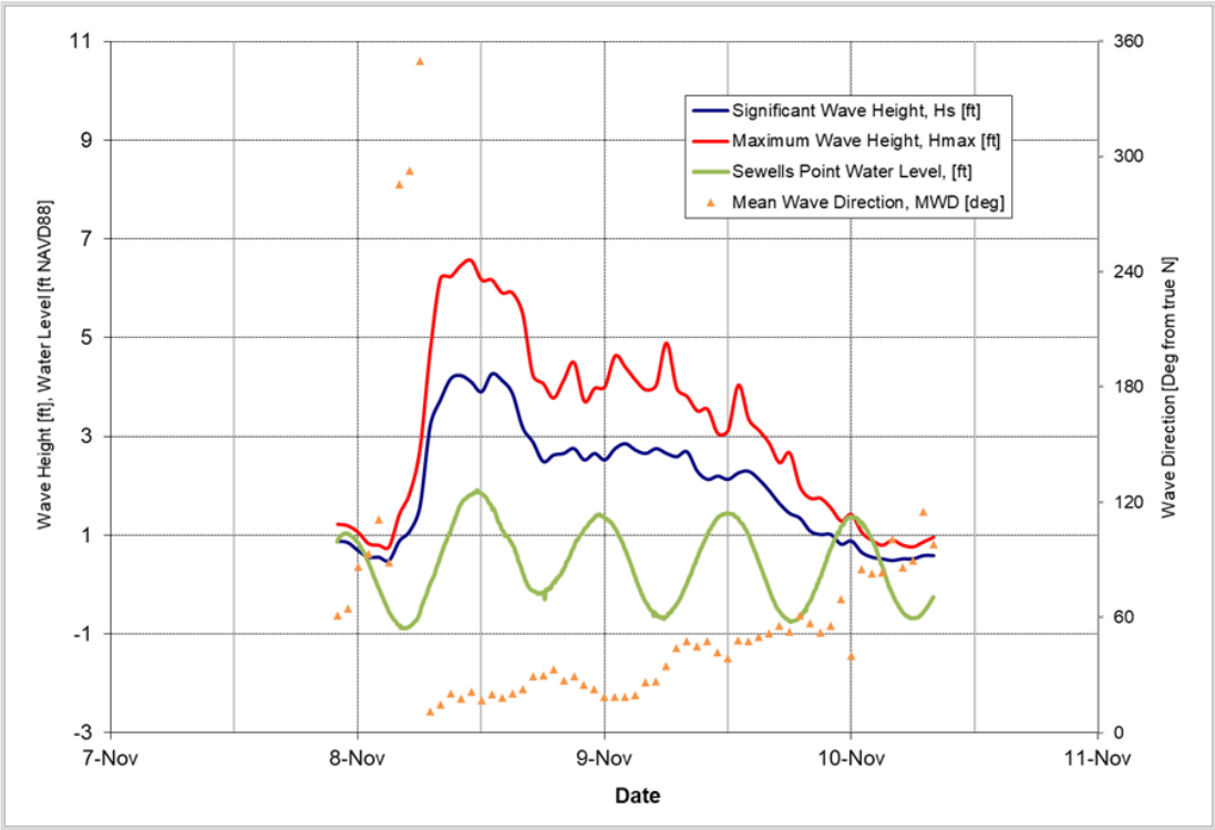
Figure 5-2: November 8, 2019 Storm
