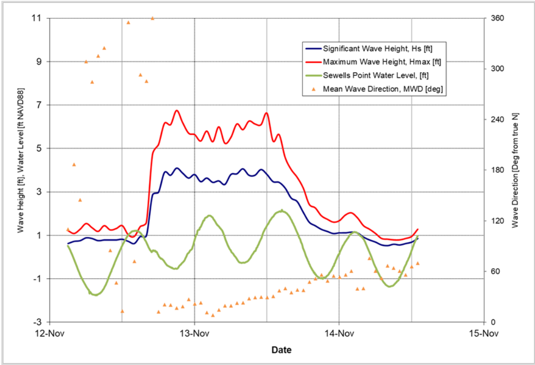
Figure 5-3: November 12, 2019 Storm
