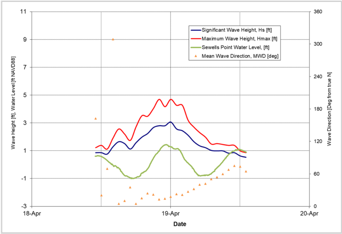
Figure 5-15: April 19, 2020 Storm
