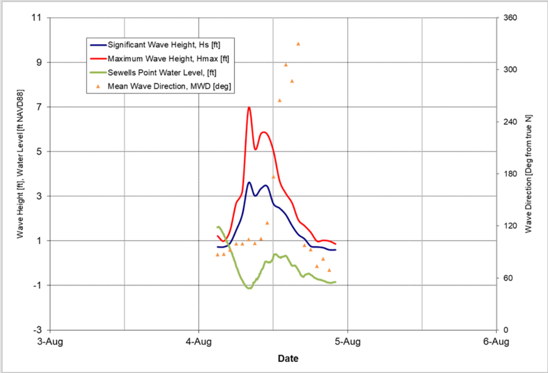
Figure 5-25: August 4, 2020 Storm
