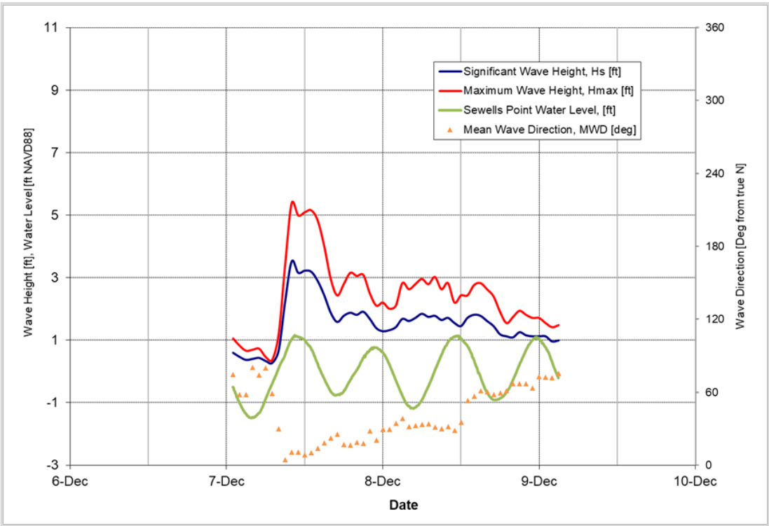
Figure 5-6: December 7, 2019 Storm
