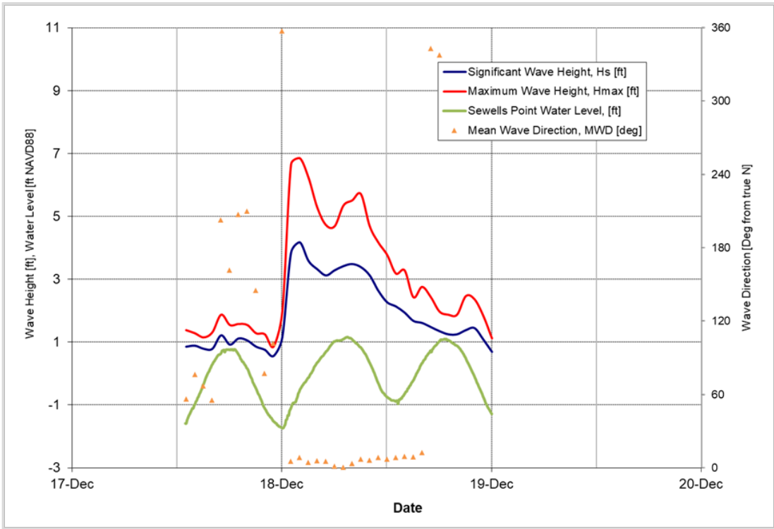
Figure 5-8: December 18, 2019 Storm
