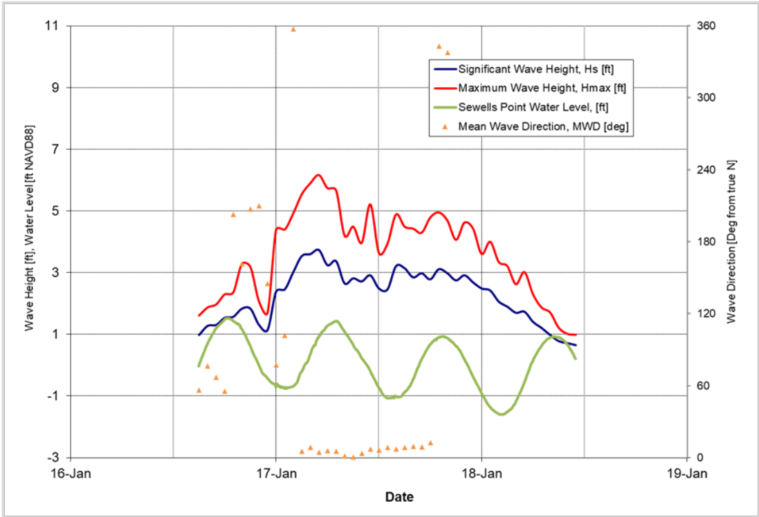
Figure 5-9: January 17, 2020 Storm
