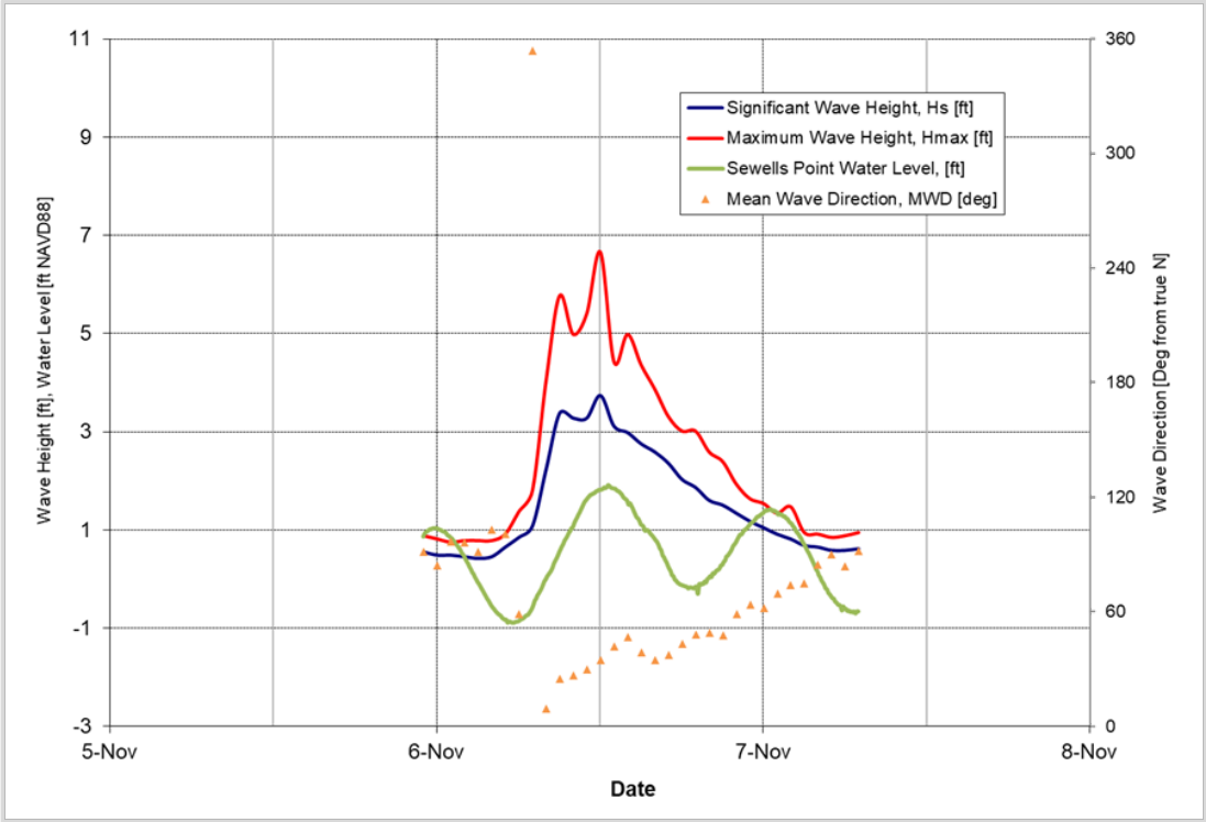
Figure 5-1: November 6, 2019 Storm
