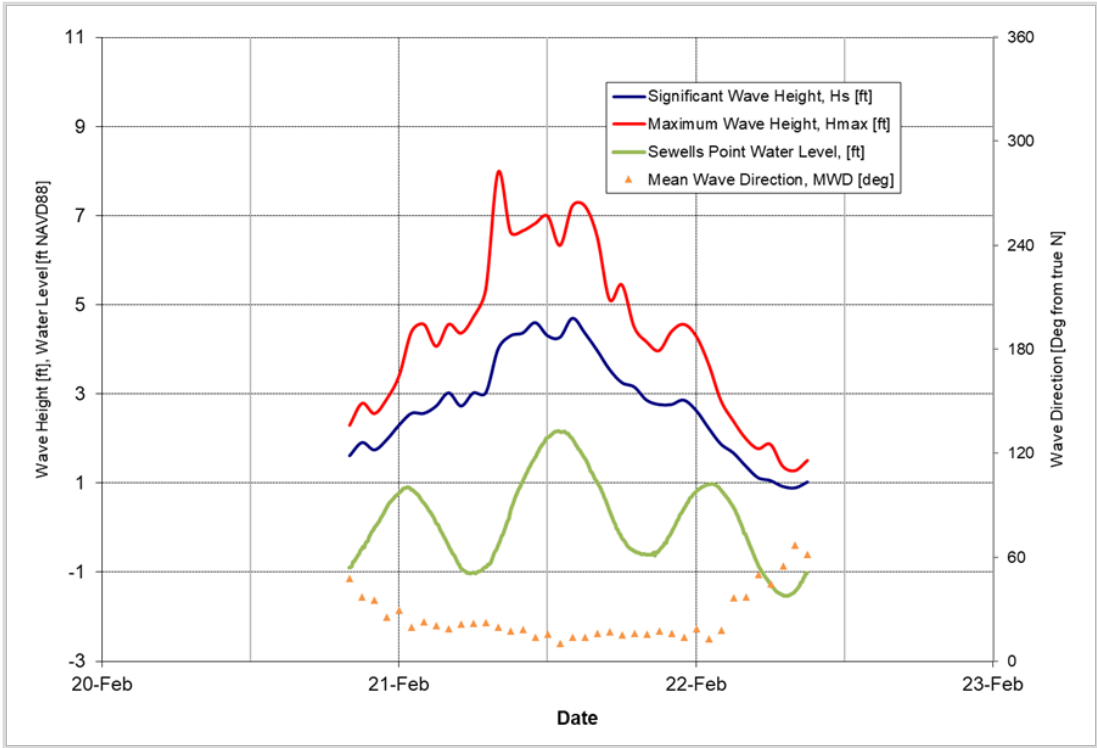
Figure 5-13: February 21, 2020 Storm
