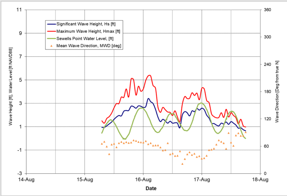
Figure 5-26: August 16, 2020 Storm
