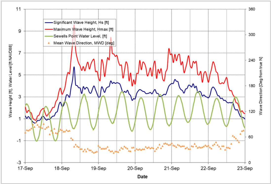
Figure 5-29: September 18, 2020 Storm
