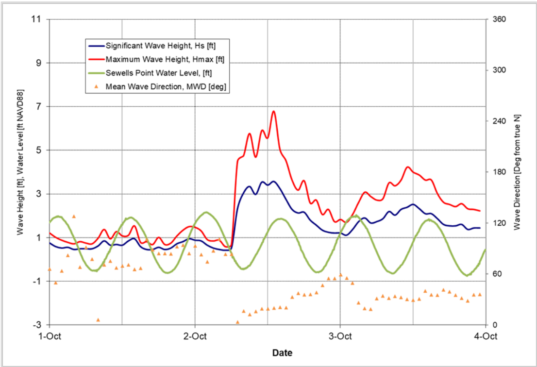
Figure 5-30: October 2, 2020 Storm
