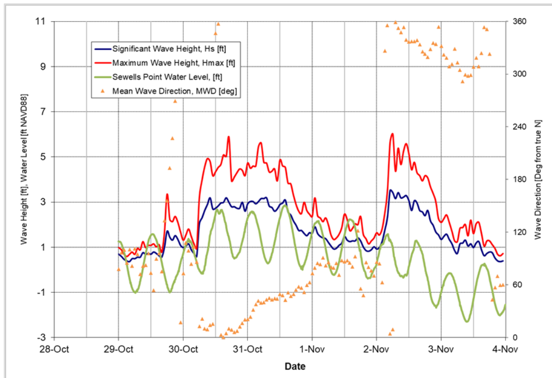
Figure 5-33: October 30, 2020 Storm
