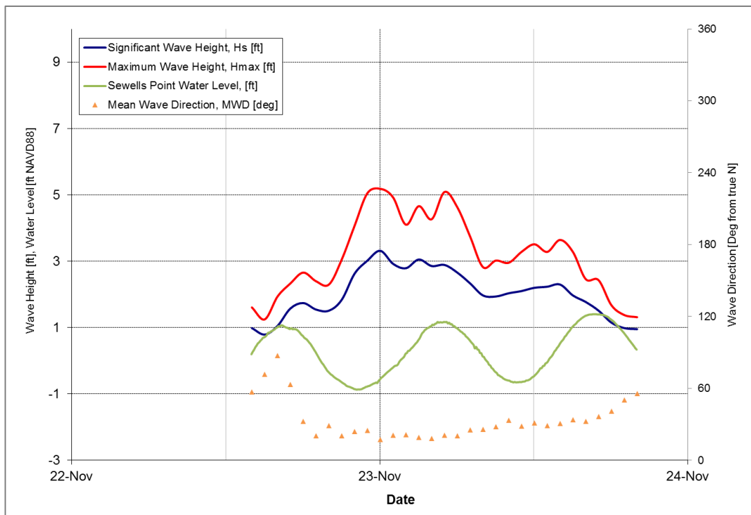
Figure 5-6: November 22, 2017 Storm
