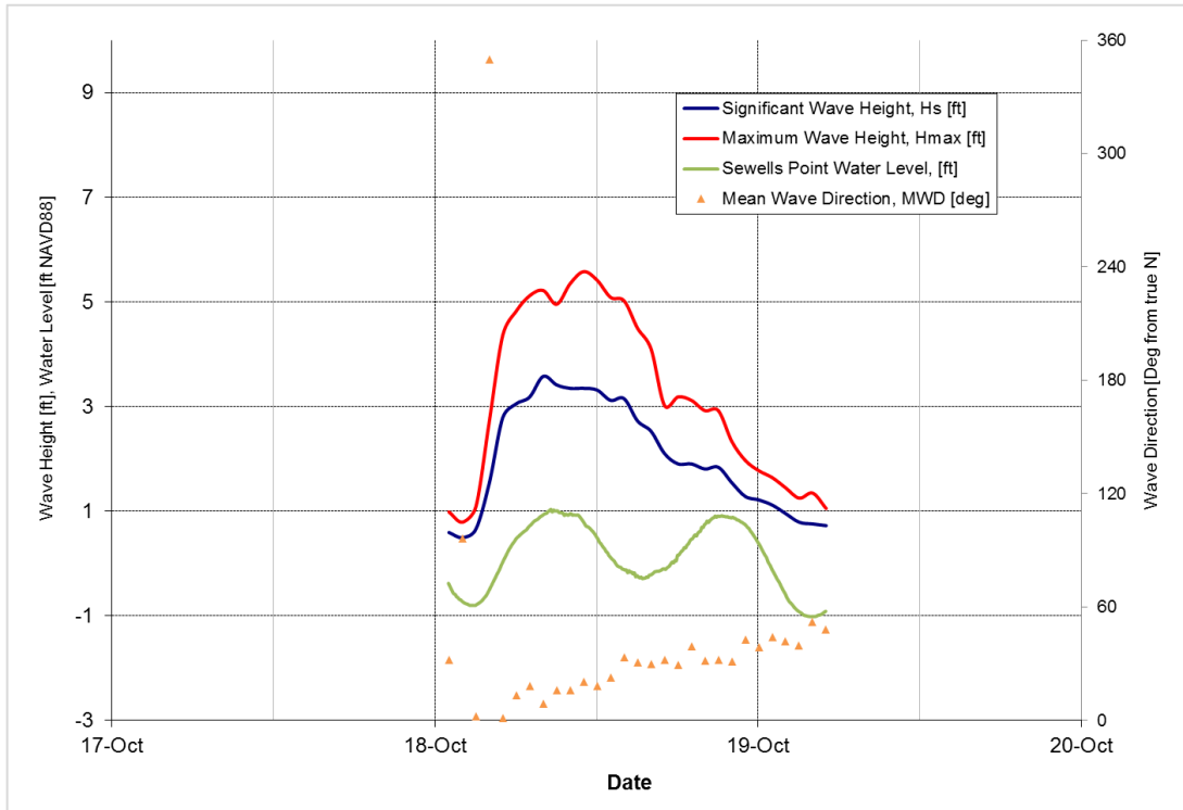
Figure 5-33: October 18, 2018 Storm
