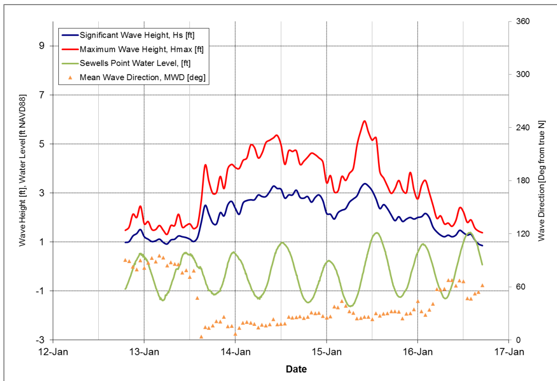
Figure 5-14: January 14, 2018 Storm
