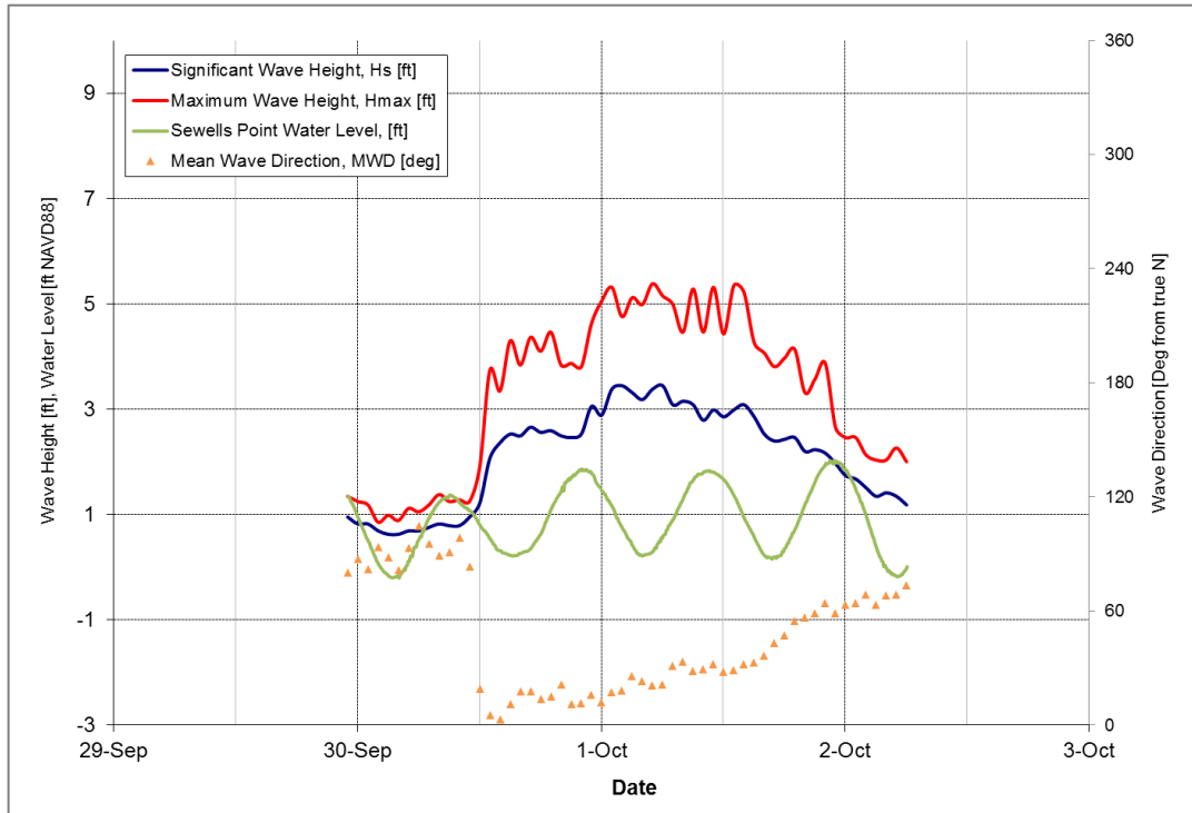
Figure 5-1: October 1, 2017 Storm
