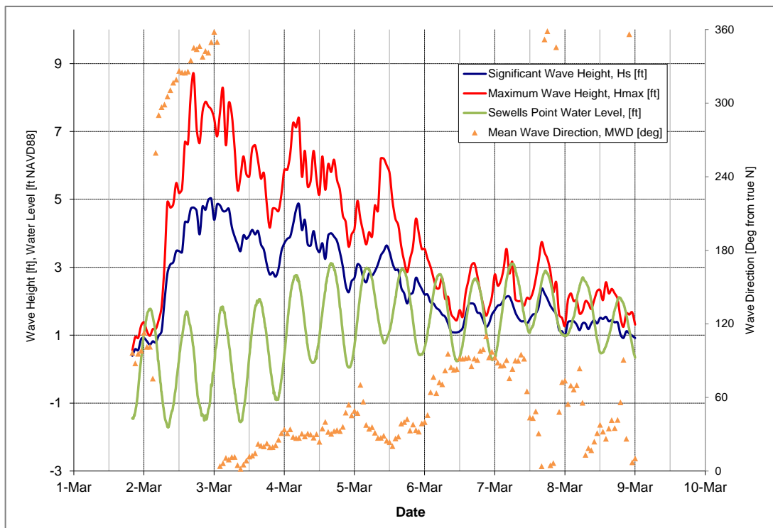
Figure 5-20: March 2, 2018 Storm
