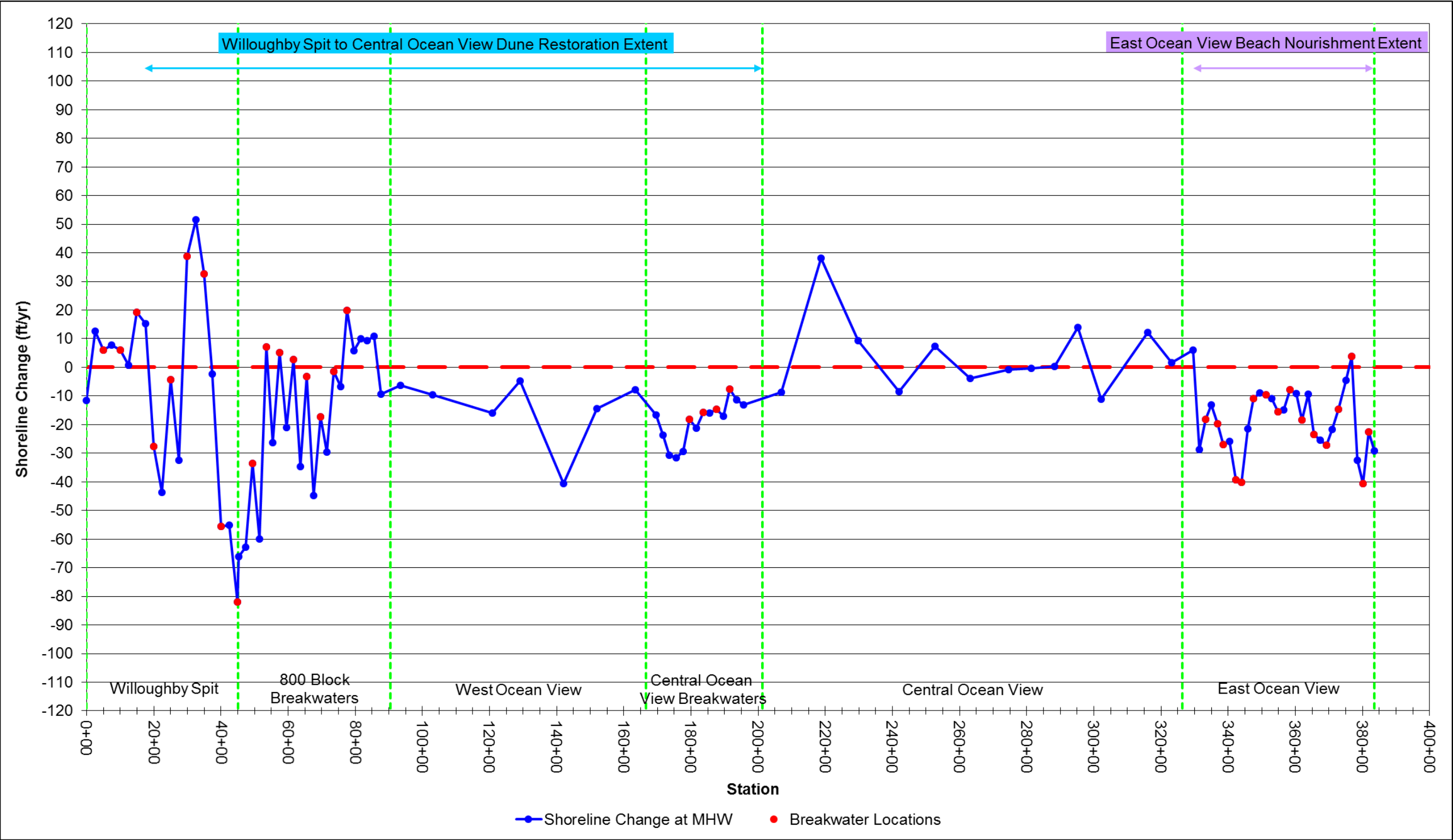
Figure 5-37: Shoreline Change Rate (ft/yr) at Mean High Water (+0.98 ft NAVD88) for October 2017 to November 2018 (Note: Positive = Accretion, Negative = Erosion)
