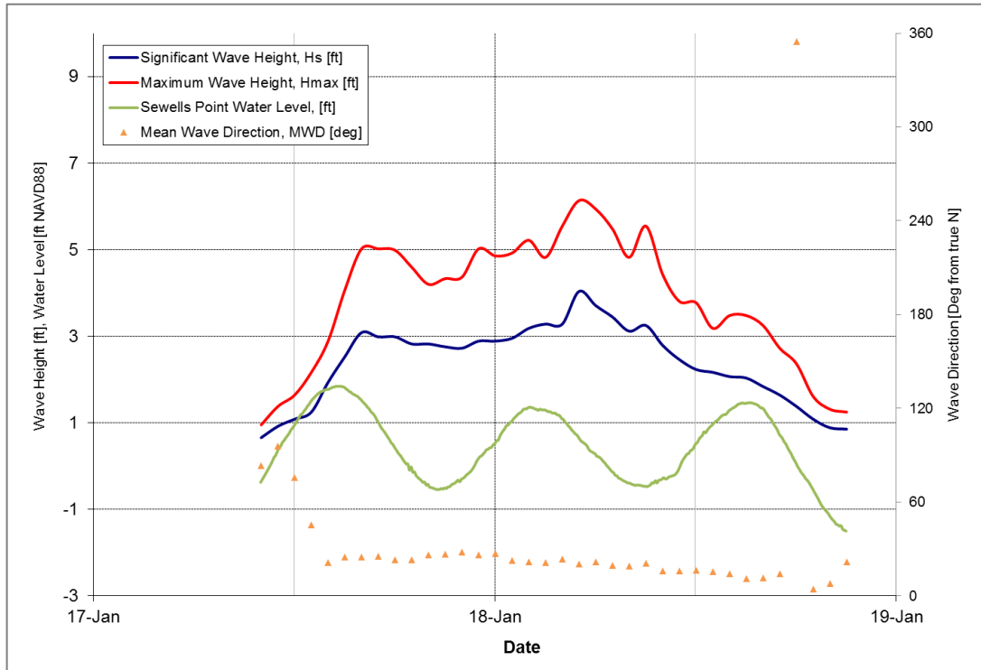
Figure 5-15: January 18, 2018 Storm
