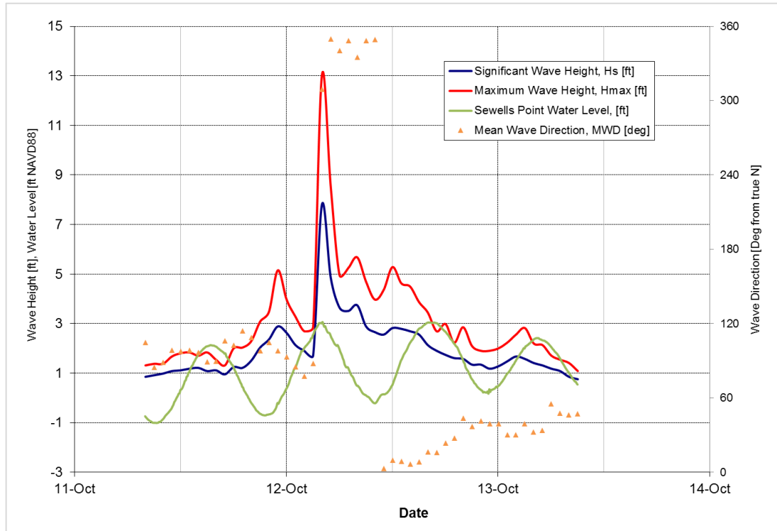
Figure 5-31: October 12, 2018 Storm
