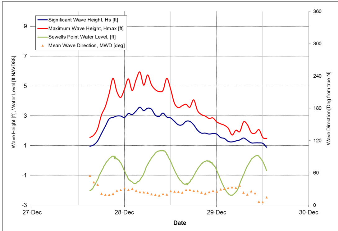
Figure 5-11: December 28, 2017 Storm
