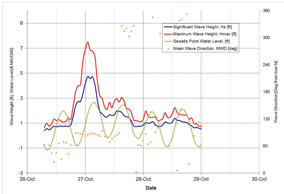
Figure 5-36: October 27, 2018 Storm
