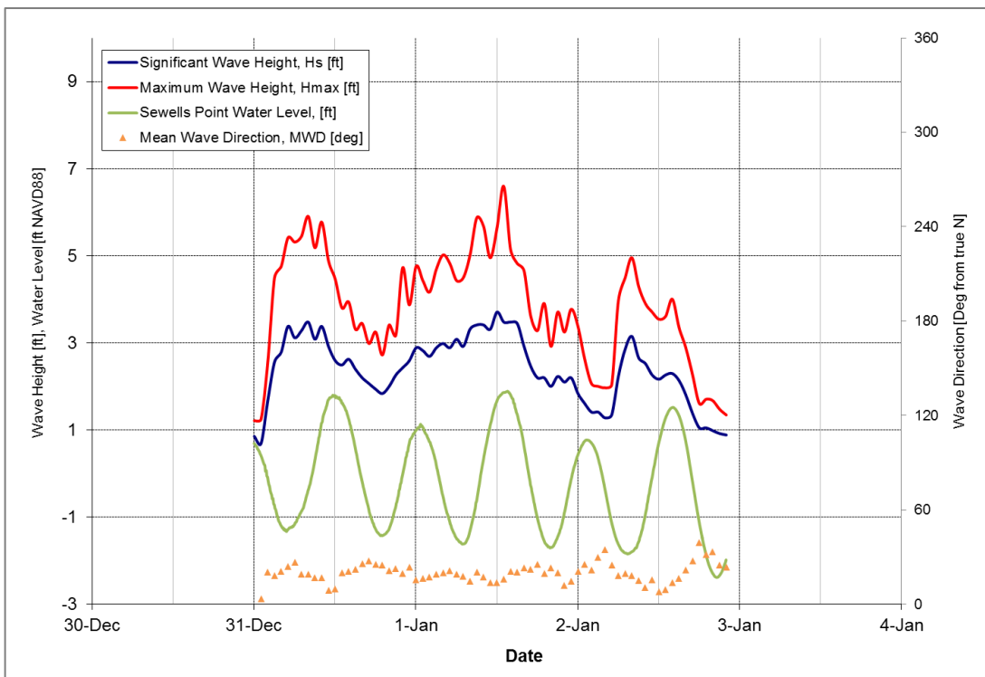
Figure 5-12: December 31, 2017 Storm
