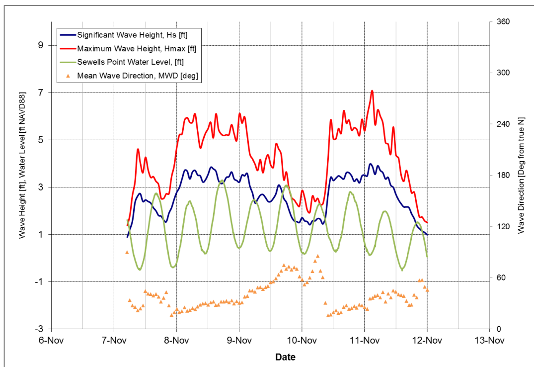
Figure 5-4: November 8, 2017 Storm
