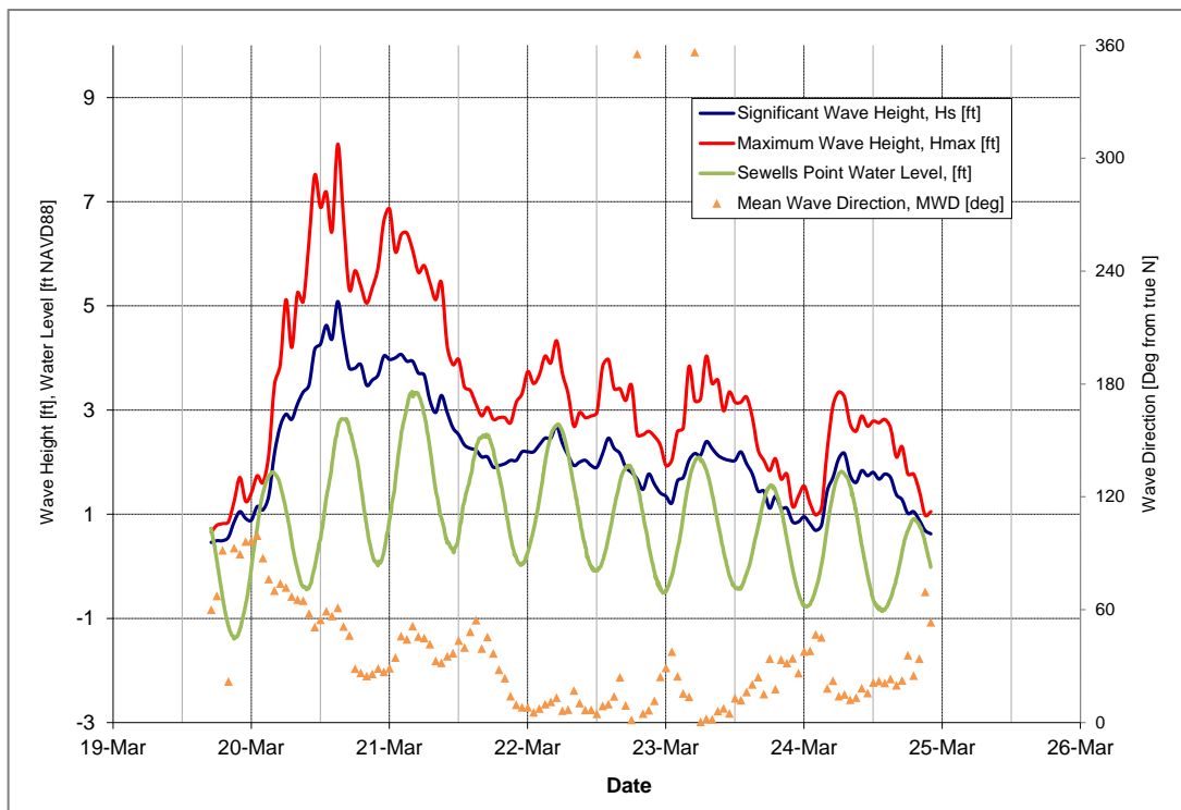
Figure 5-22: March 20, 2018 Storm
