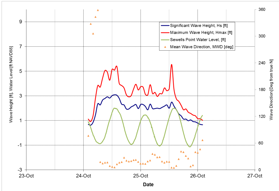
Figure 5-35: October 24, 2018 Storm
