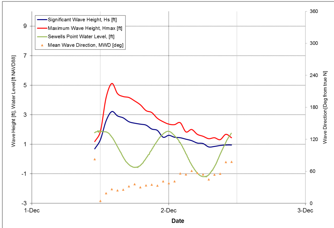
Figure 5-7: December 1, 2017 Storm
