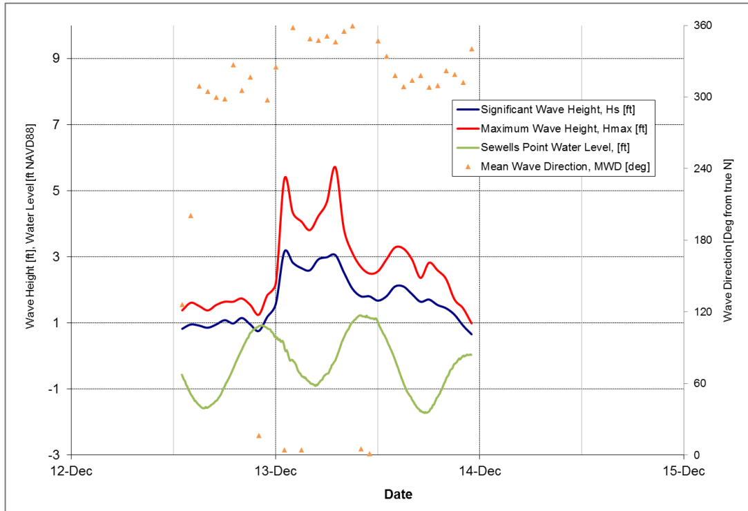
Figure 5-9: December 13, 2017 Storm
