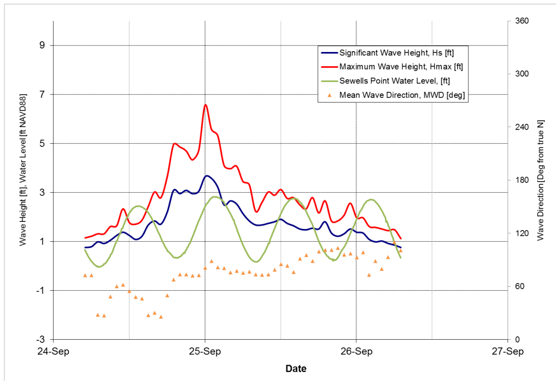
Figure 5-30: September 24, 2018 Storm
