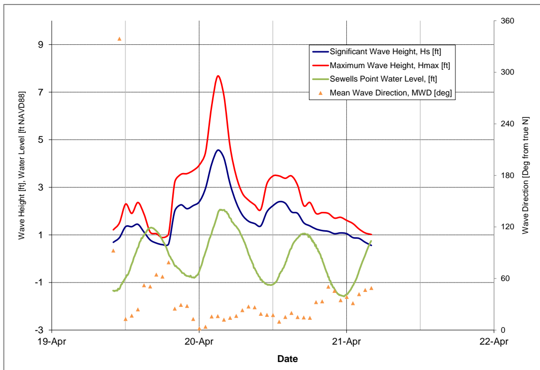
Figure 5-26: April 20, 2018 Storm
