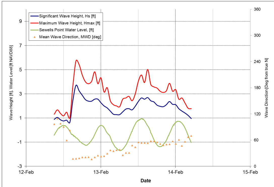
Figure 5-19: February 12, 2018 Storm
