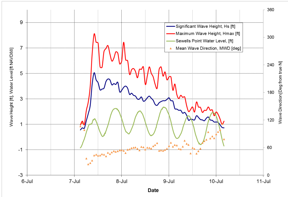
Figure 5-27: July 7, 2018 Storm
