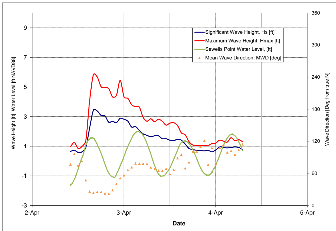
Figure 5-24: April 2, 2018 Storm
