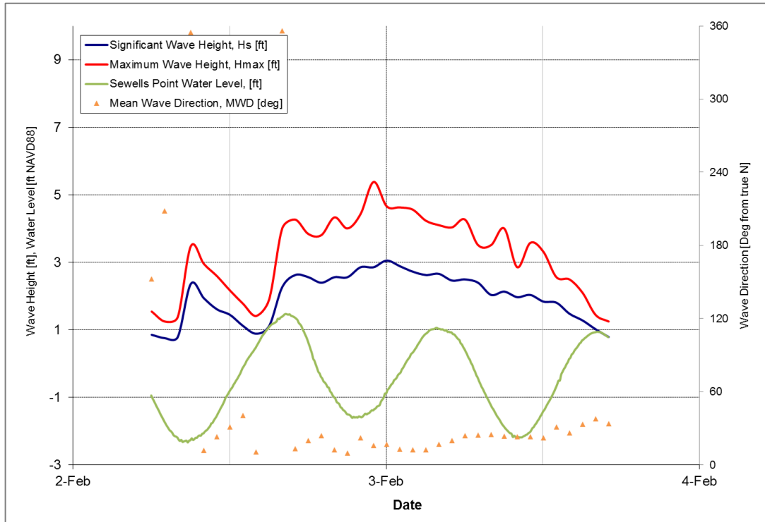
Figure 5-17: February 3, 2018 Storm
