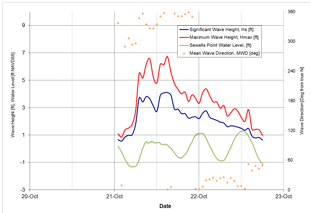
Figure 5-34: October 21, 2018 Storm
