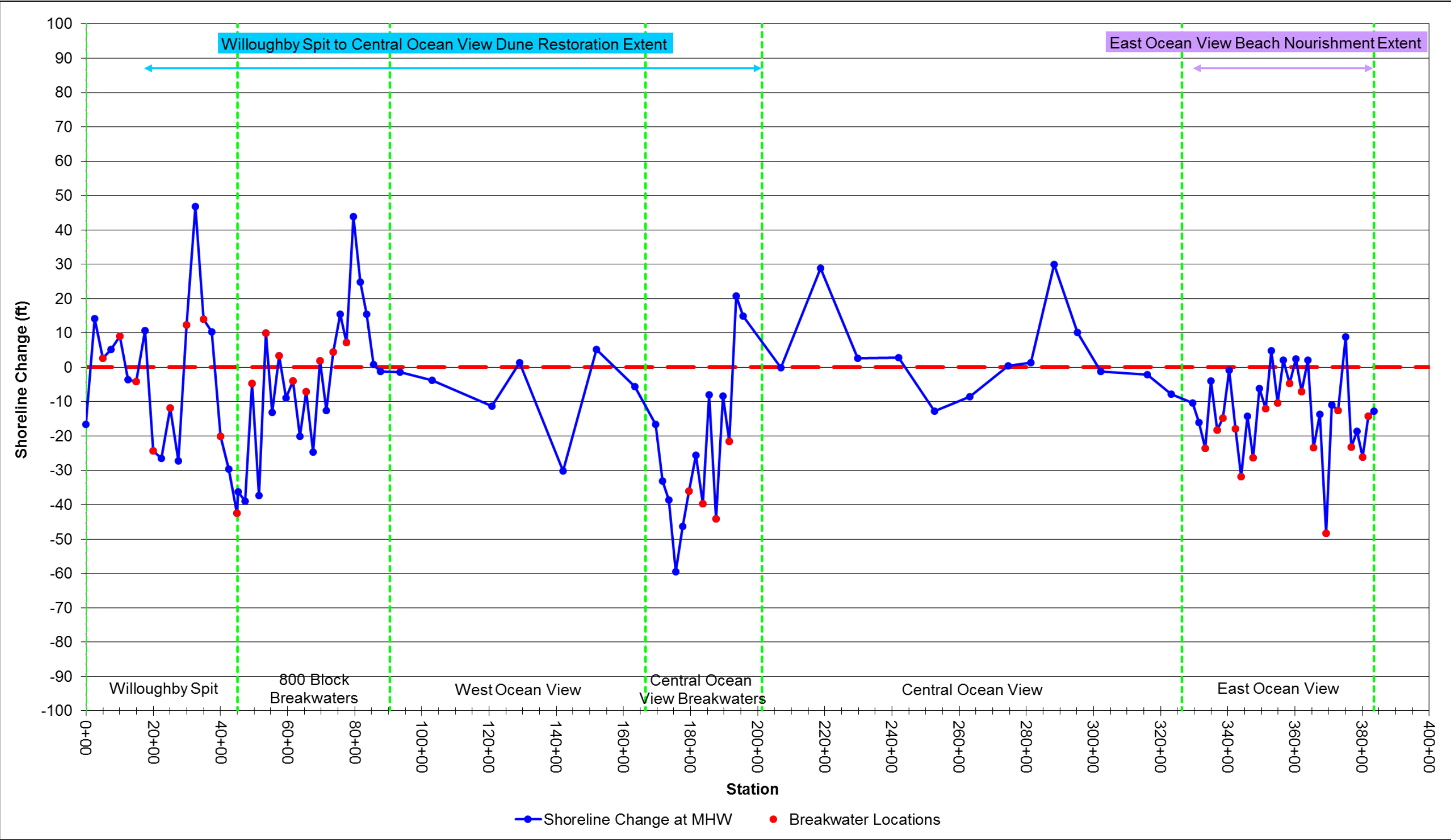
Figure 5-39: Shoreline Change (ft) at Mean High Water (+0.98 ft NAVD88) for April 2018 to November 2018 (Note: Positive = Accretion, Negative = Erosion)
