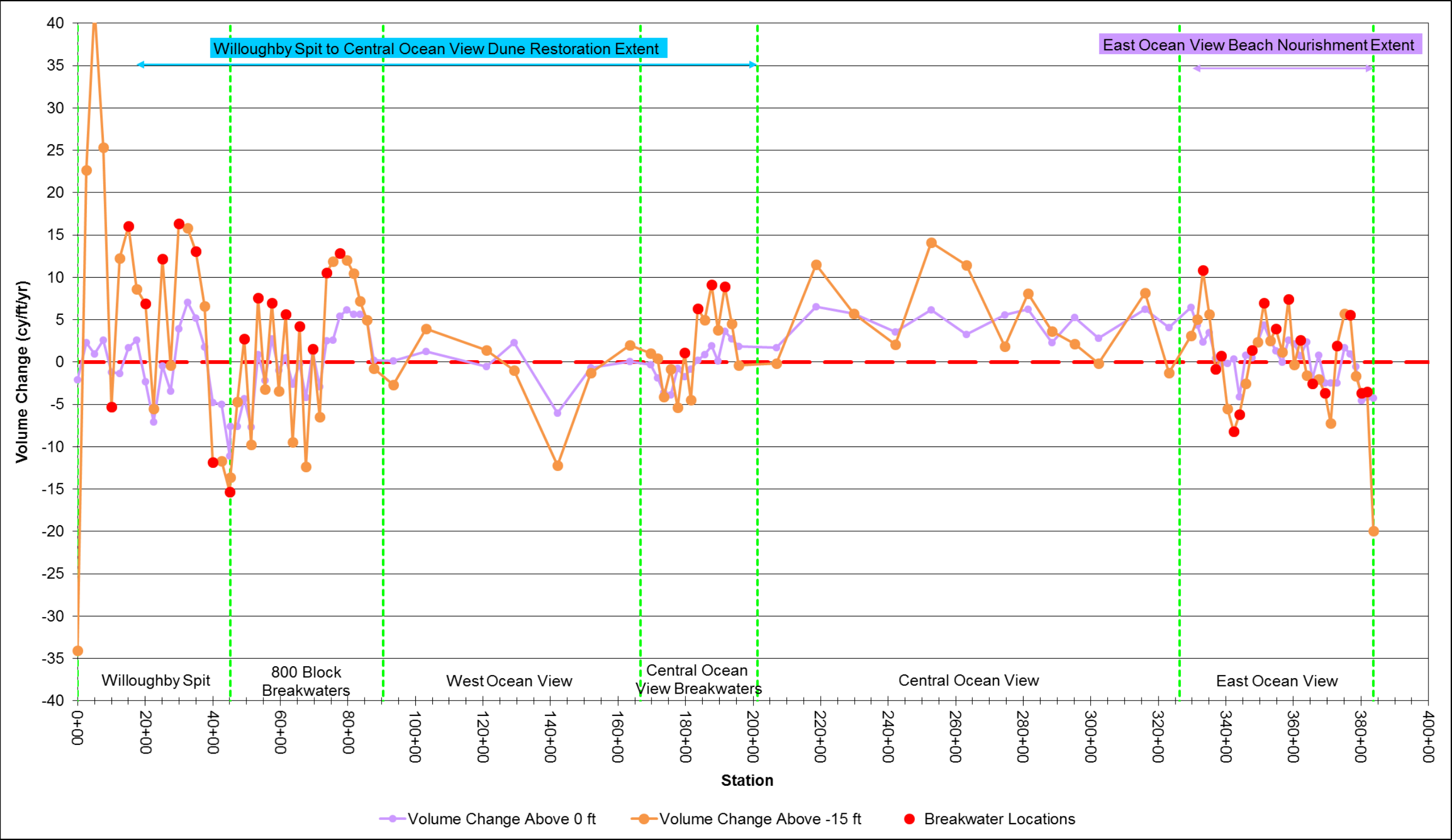
Figure 5-38: Volume Change Rate above 0 ft NAVD88 and -15 ft NAVD88 (cy/ft/yr) for October 2017 to November 2018 (Note: Positive = Accretion, Negative = Erosion)
