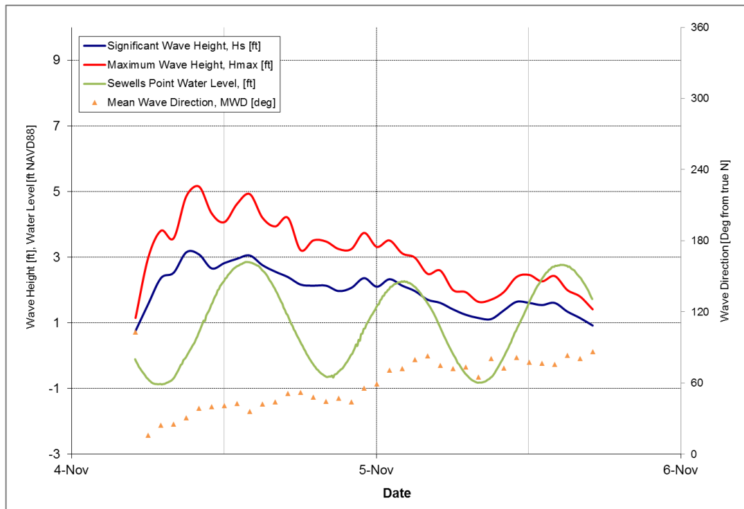
Figure 5-3: November 4, 2017 Storm
