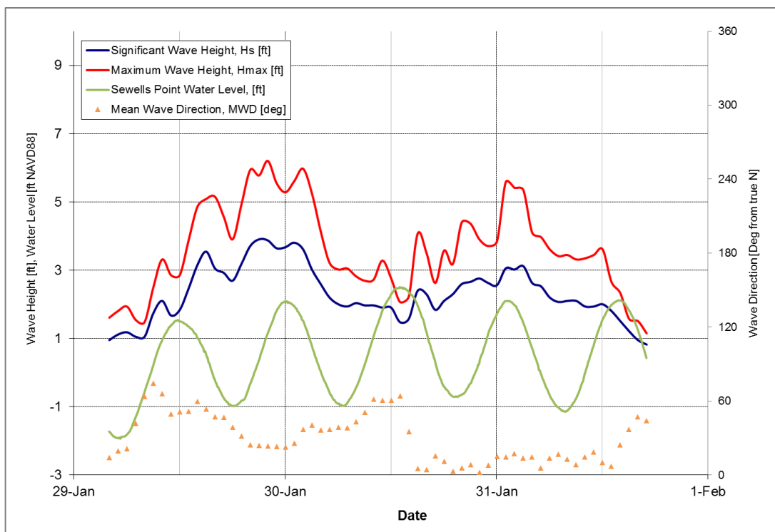
Figure 5-16: January 29, 2018 Storm
