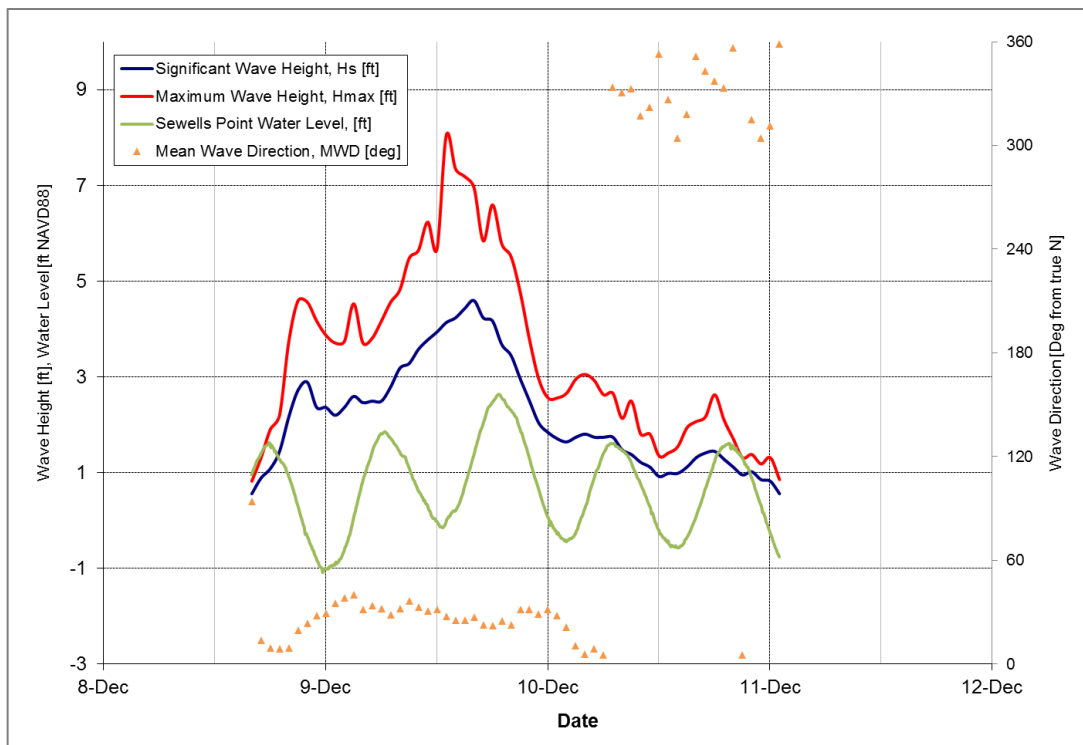
Figure 5-8: December 9, 2017 Storm
