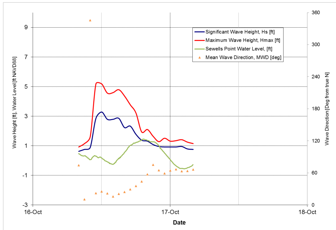
Figure 5-32: October 16, 2018 Storm
