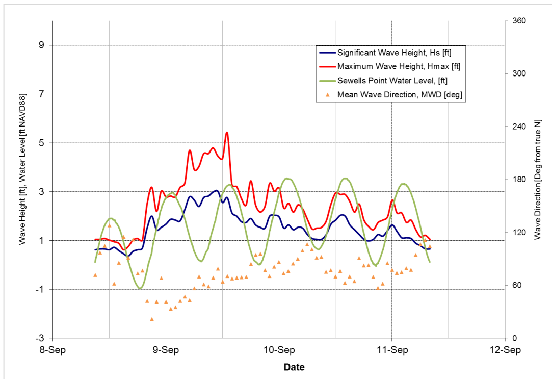
Figure 5-28: September 9, 2018 Storm
