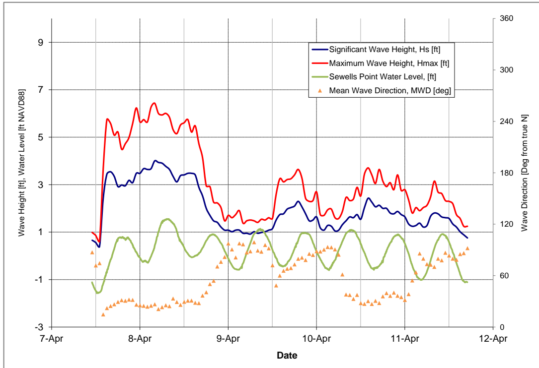
Figure 5-25: April 8, 2018 Storm
