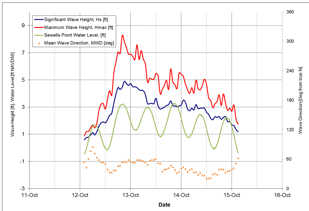
Figure 5-2: October 12, 2017 Storm
