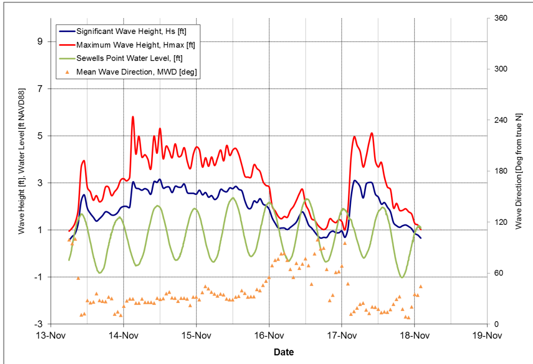
Figure 5-5: November 14, 2017 Storm
