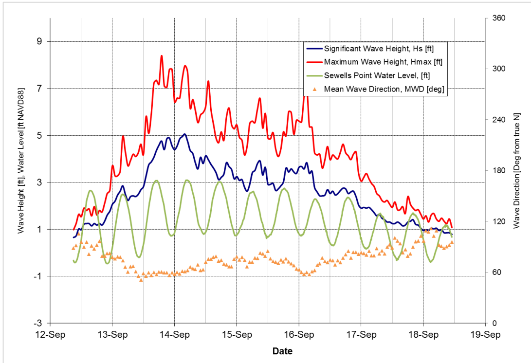
Figure 5-29: September 14, 2018 Storm
