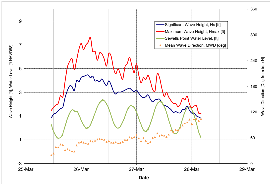
Figure 5-23: March 26, 2018 Storm
