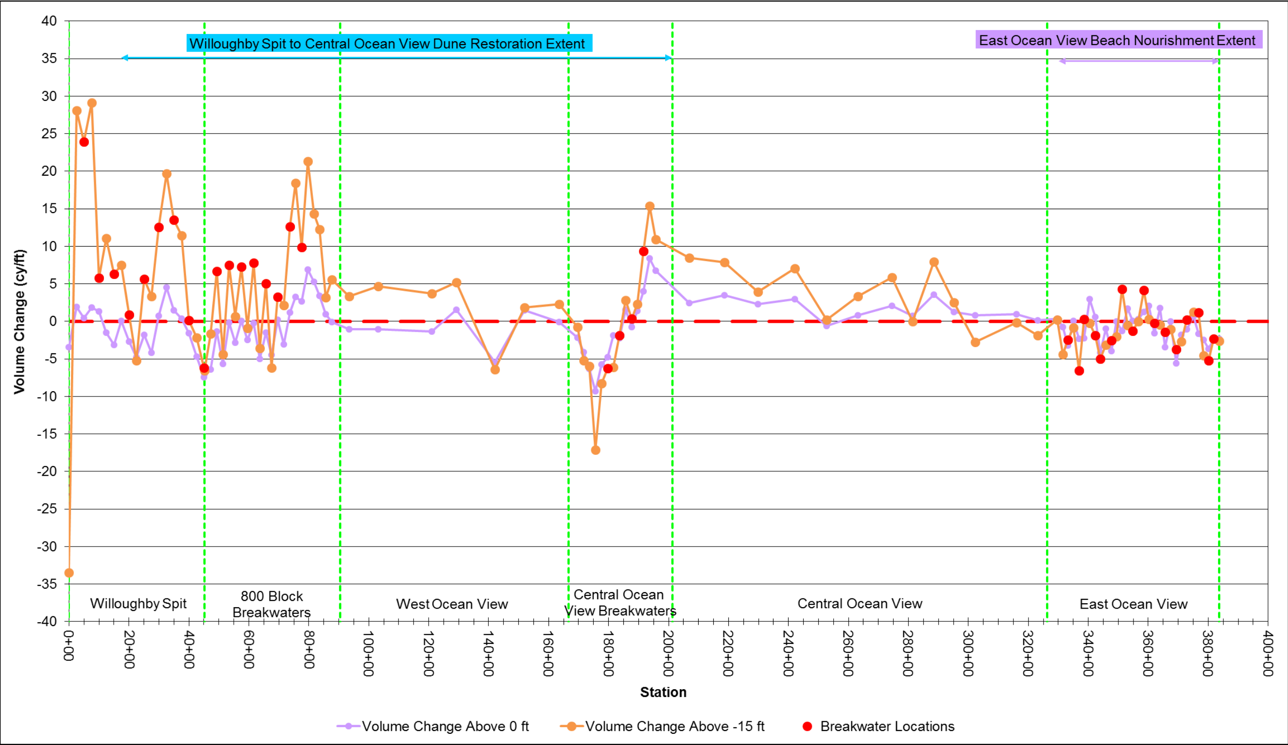
Figure 5-40: Volume Change Above 0 ft NAVD88 and -15 ft NAVD88 (cy/ft) for April 2018 to November 2018 (Note: Positive = Accretion, Negative = Erosion)
