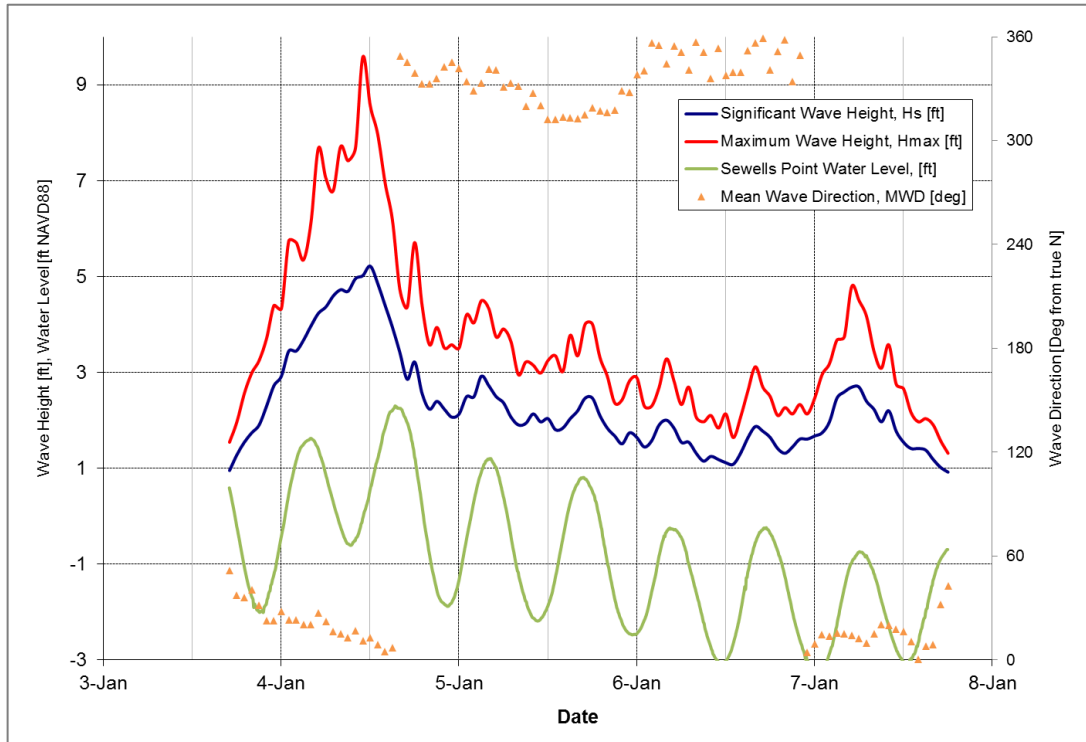
Figure 5-13: January 4, 2018 Storm
