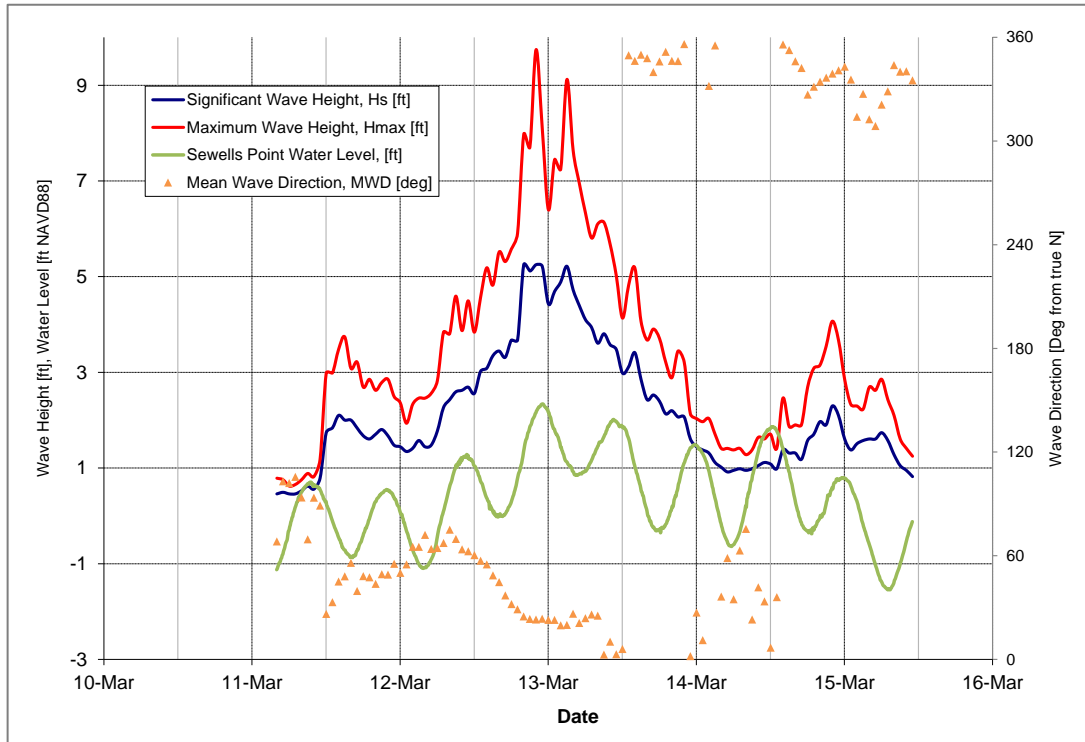
Figure 5-21: March 12, 2018 Storm
