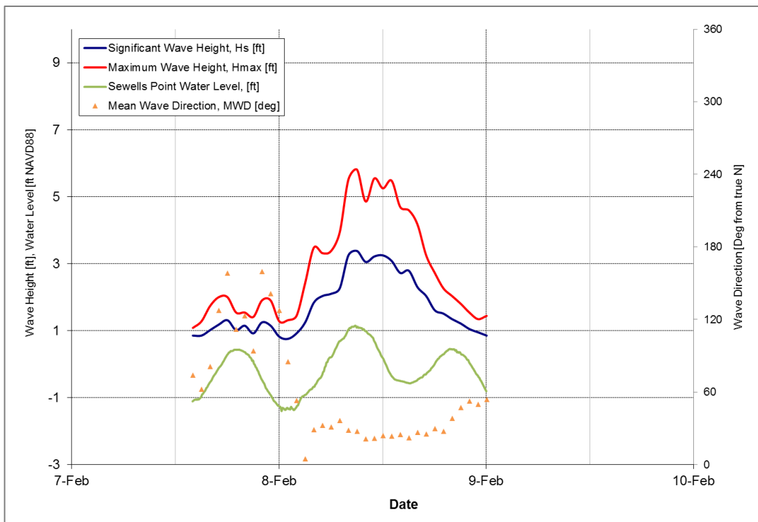
Figure 5-18: February 8, 2018 Storm
