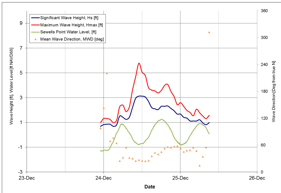
Figure 5-10: December 24, 2017 Storm
